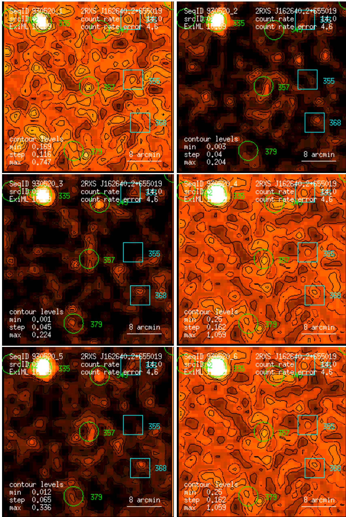
Figure 357: RASS 930520: detection 0357: band rate images, Gaussian filter: (1) PSPC channels 11 – 41, (2) 52 – 90, (3) 91 – 201, (4) 11 – 235, (5) 52 – 201, (6) 11 – 201. Broad band rates in counts/ks. Band rate contour levels in counts/ks/arcmin 2 .
