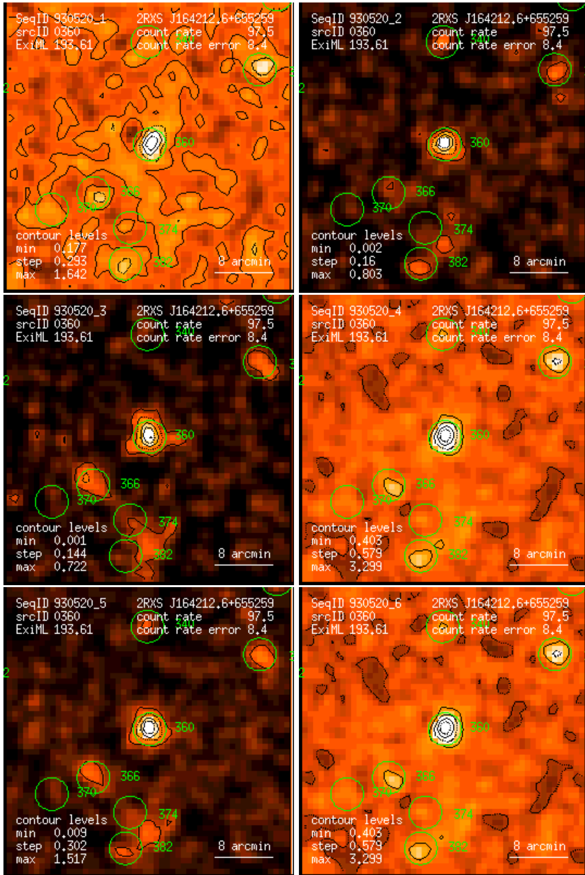
Figure 360: RASS 930520: detection 0360: band rate images, Gaussian filter: (1) PSPC channels 11 – 41, (2) 52 – 90, (3) 91 – 201, (4) 11 – 235, (5) 52 – 201, (6) 11 – 201. Broad band rates in counts/ks. Band rate contour levels in counts/ks/arcmin 2 .
