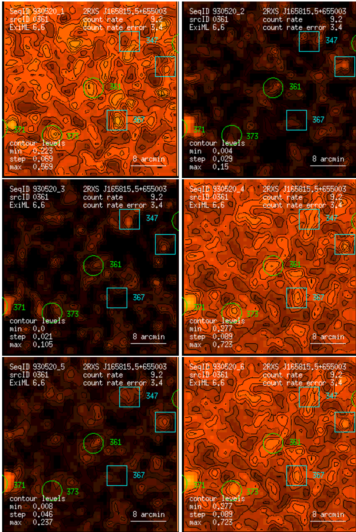
Figure 361: RASS 930520: detection 0361: band rate images, Gaussian filter: (1) PSPC channels 11 – 41, (2) 52 – 90, (3) 91 – 201, (4) 11 – 235, (5) 52 – 201, (6) 11 – 201. Broad band rates in counts/ks. Band rate contour levels in counts/ks/arcmin 2 .
