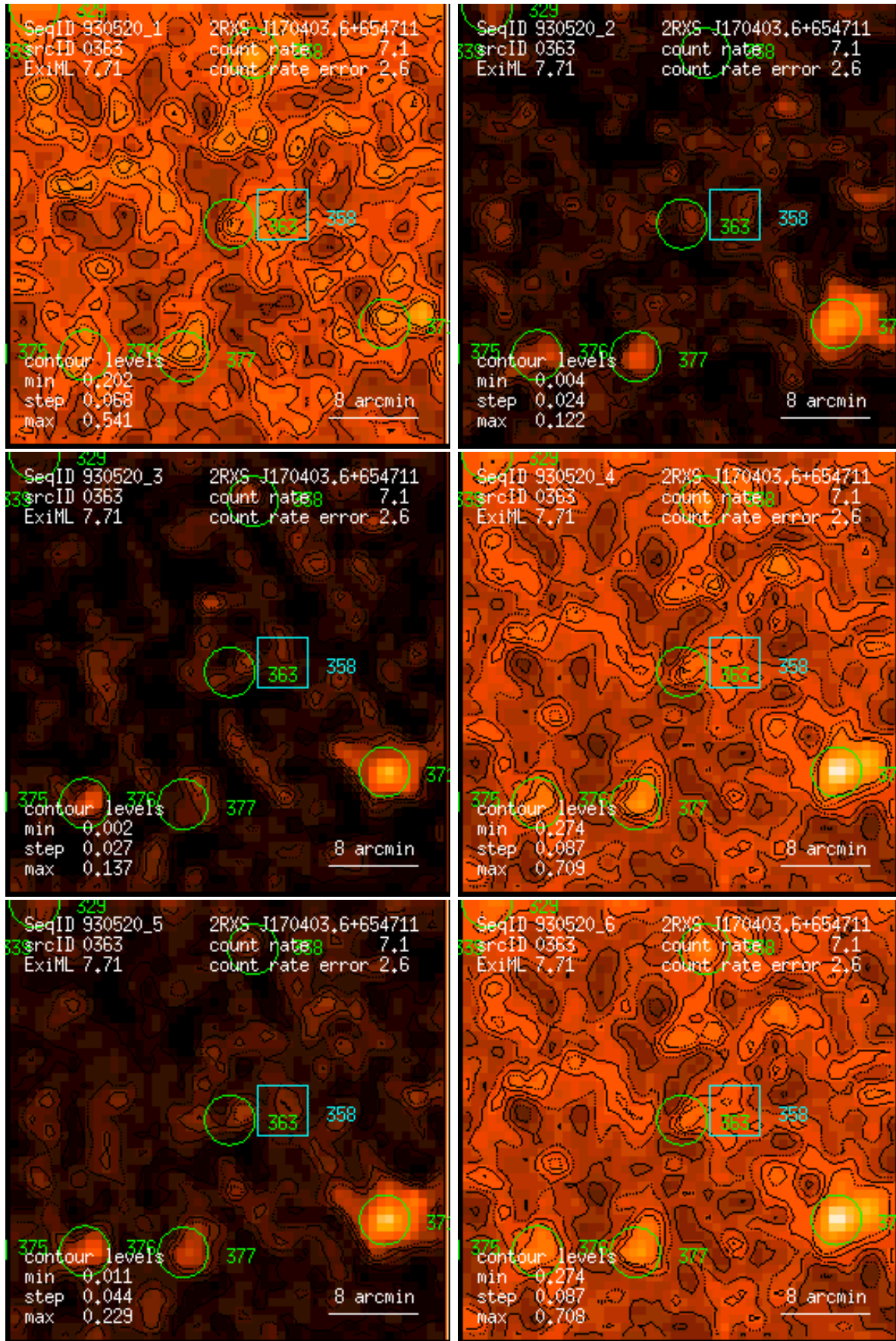
Figure 363: RASS 930520: detection 0363: band rate images, Gaussian filter: (1) PSPC channels 11 – 41, (2) 52 – 90, (3) 91 – 201, (4) 11 – 235, (5) 52 – 201, (6) 11 – 201. Broad band rates in counts/ks. Band rate contour levels in counts/ks/arcmin 2 .
