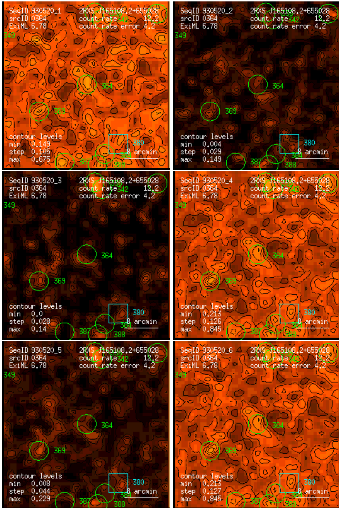
Figure 364: RASS 930520: detection 0364: band rate images, Gaussian filter: (1) PSPC channels 11 – 41, (2) 52 – 90, (3) 91 – 201, (4) 11 – 235, (5) 52 – 201, (6) 11 – 201. Broad band rates in counts/ks. Band rate contour levels in counts/ks/arcmin 2 .
