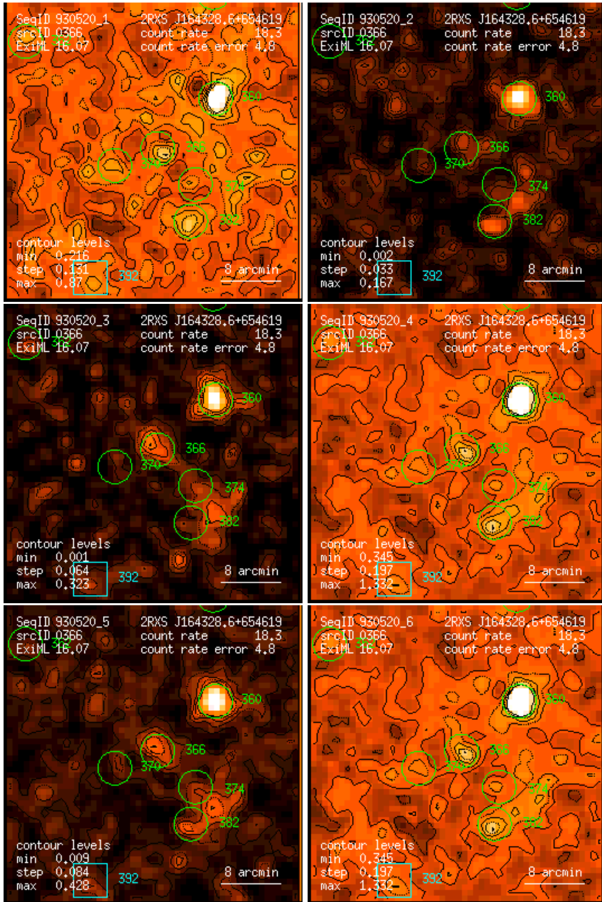
Figure 366: RASS 930520: detection 0366: band rate images, Gaussian filter: (1) PSPC channels 11 – 41, (2) 52 – 90, (3) 91 – 201, (4) 11 – 235, (5) 52 – 201, (6) 11 – 201. Broad band rates in counts/ks. Band rate contour levels in counts/ks/arcmin 2 .
