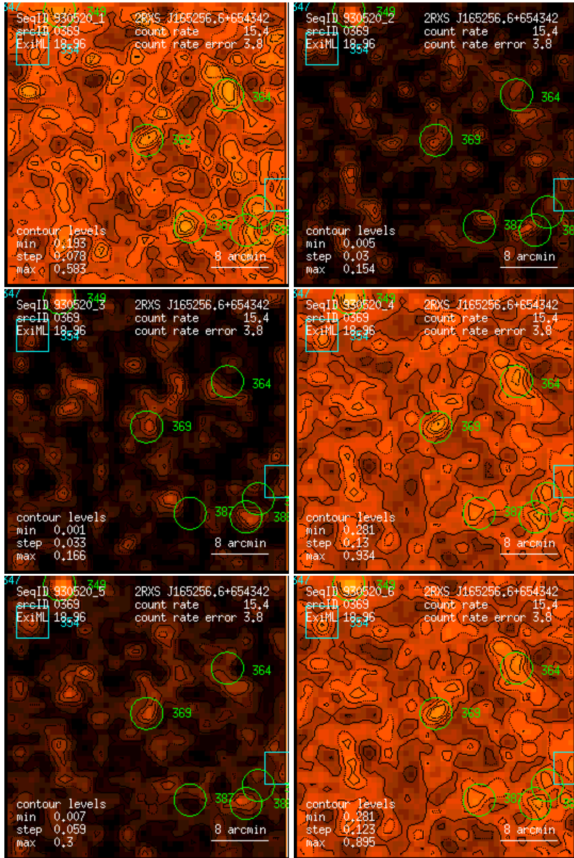
Figure 369: RASS 930520: detection 0369: band rate images, Gaussian filter: (1) PSPC channels 11 – 41, (2) 52 – 90, (3) 91 – 201, (4) 11 – 235, (5) 52 – 201, (6) 11 – 201. Broad band rates in counts/ks. Band rate contour levels in counts/ks/arcmin 2 .
