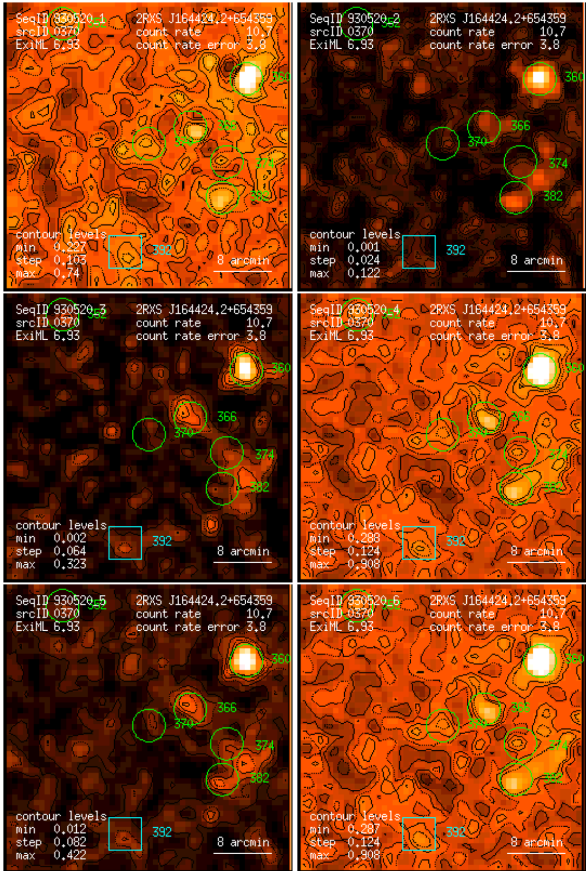
Figure 370: RASS 930520: detection 0370: band rate images, Gaussian filter: (1) PSPC channels 11 – 41, (2) 52 – 90, (3) 91 – 201, (4) 11 – 235, (5) 52 – 201, (6) 11 – 201. Broad band rates in counts/ks. Band rate contour levels in counts/ks/arcmin 2 .
