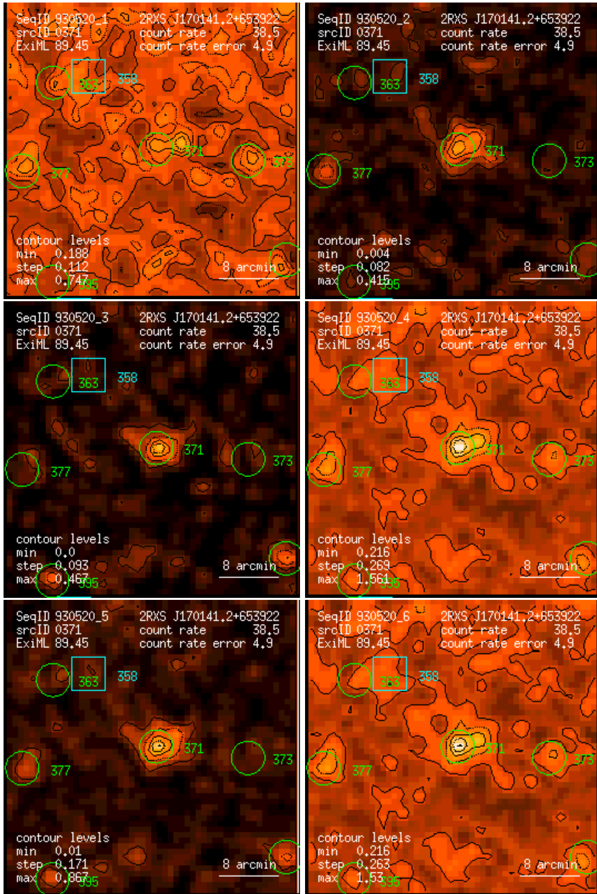
Figure 371: RASS 930520: detection 0371: band rate images, Gaussian filter: (1) PSPC channels 11 – 41, (2) 52 – 90, (3) 91 – 201, (4) 11 – 235, (5) 52 – 201, (6) 11 – 201. Broad band rates in counts/ks. Band rate contour levels in counts/ks/arcmin 2 .
