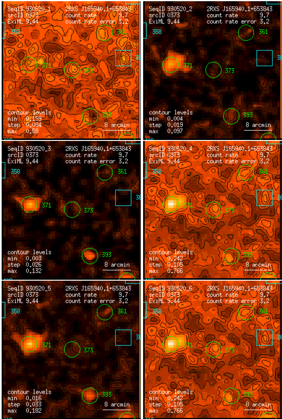
Figure 373: RASS 930520: detection 0373: band rate images, Gaussian filter: (1) PSPC channels 11 – 41, (2) 52 – 90, (3) 91 – 201, (4) 11 – 235, (5) 52 – 201, (6) 11 – 201. Broad band rates in counts/ks. Band rate contour levels in counts/ks/arcmin 2 .
