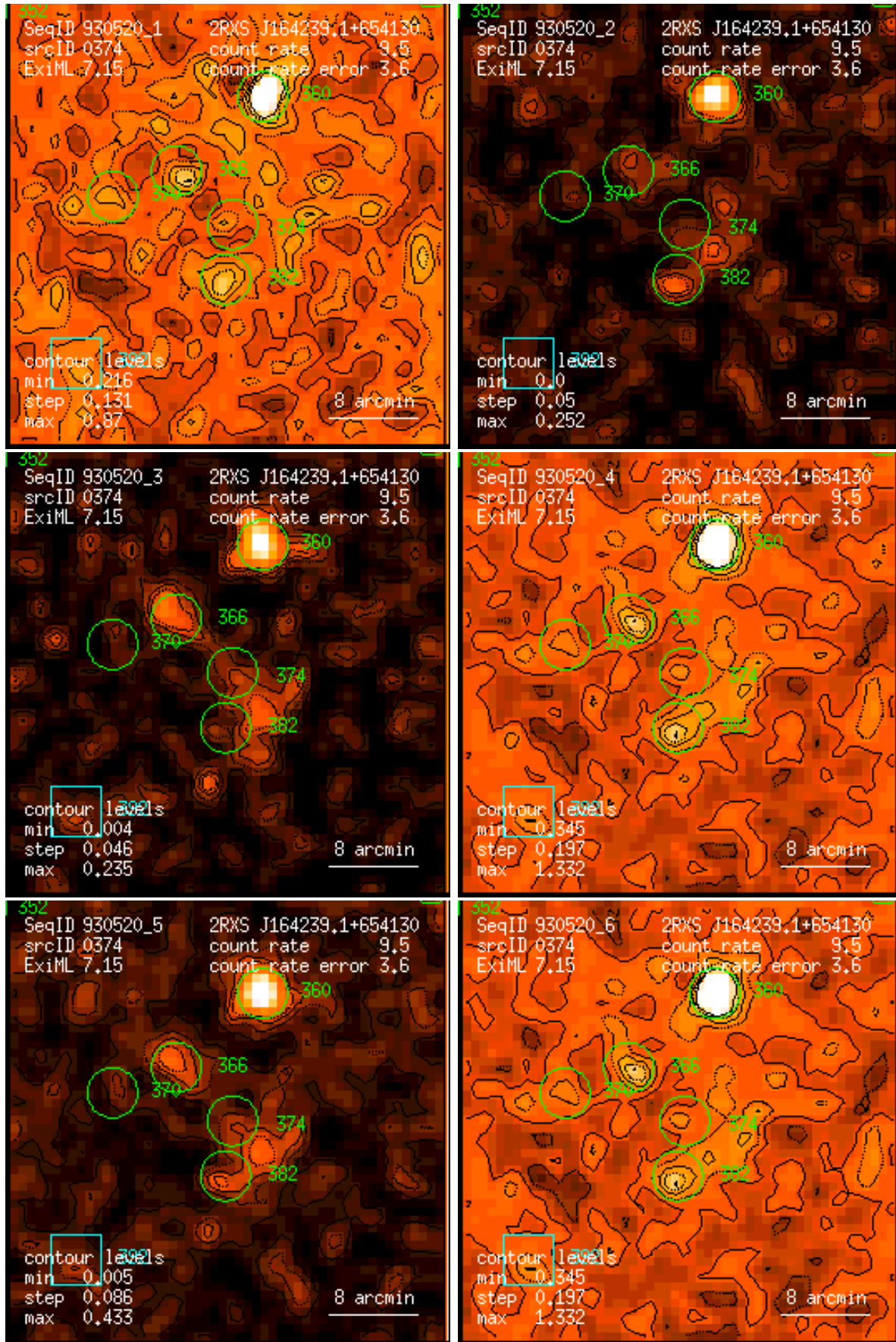
Figure 374: RASS 930520: detection 0374: band rate images, Gaussian filter: (1) PSPC channels 11 – 41, (2) 52 – 90, (3) 91 – 201, (4) 11 – 235, (5) 52 – 201, (6) 11 – 201. Broad band rates in counts/ks. Band rate contour levels in counts/ks/arcmin 2 .
