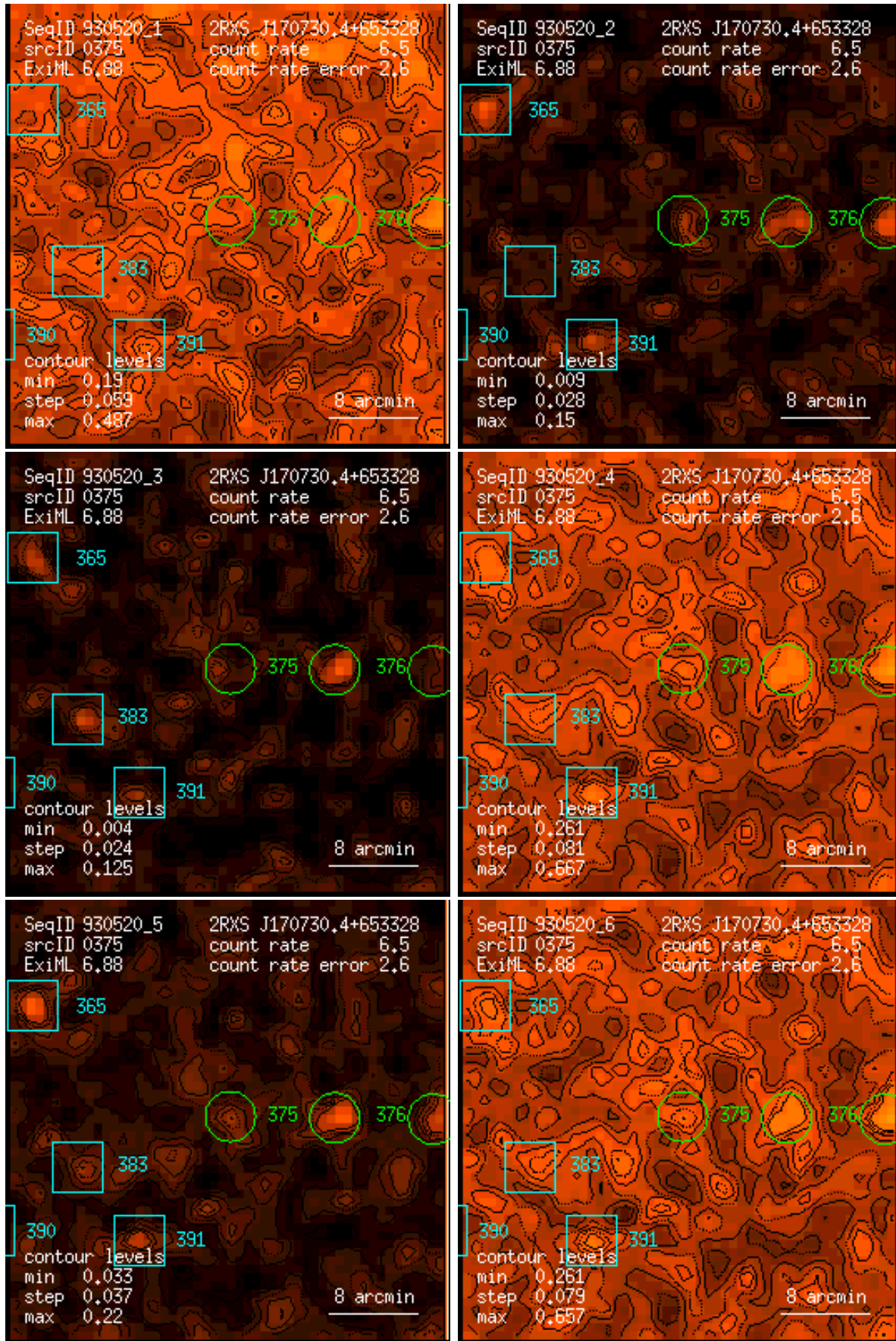
Figure 375: RASS 930520: detection 0375: band rate images, Gaussian filter: (1) PSPC channels 11 – 41, (2) 52 – 90, (3) 91 – 201, (4) 11 – 235, (5) 52 – 201, (6) 11 – 201. Broad band rates in counts/ks. Band rate contour levels in counts/ks/arcmin 2 .
