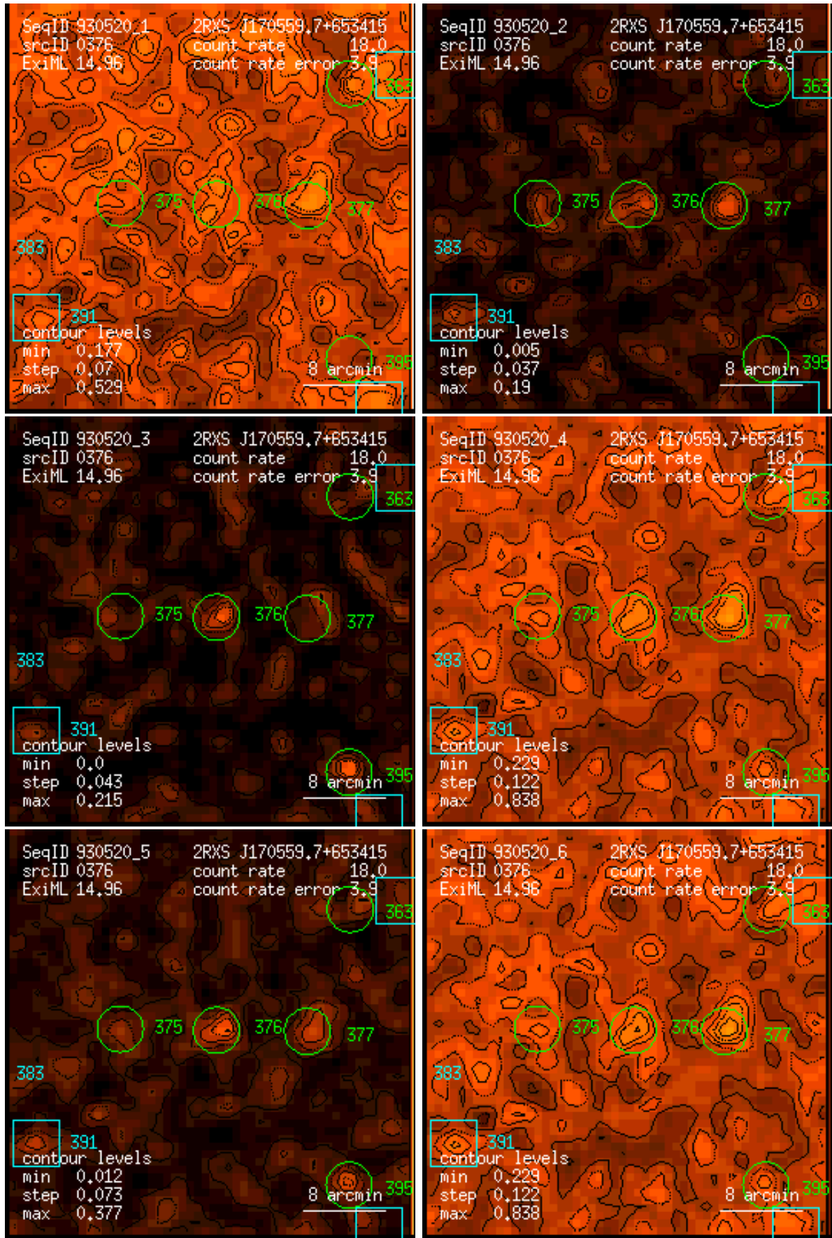
Figure 376: RASS 930520: detection 0376: band rate images, Gaussian filter: (1) PSPC channels 11 – 41, (2) 52 – 90, (3) 91 – 201, (4) 11 – 235, (5) 52 – 201, (6) 11 – 201. Broad band rates in counts/ks. Band rate contour levels in counts/ks/arcmin 2 .
