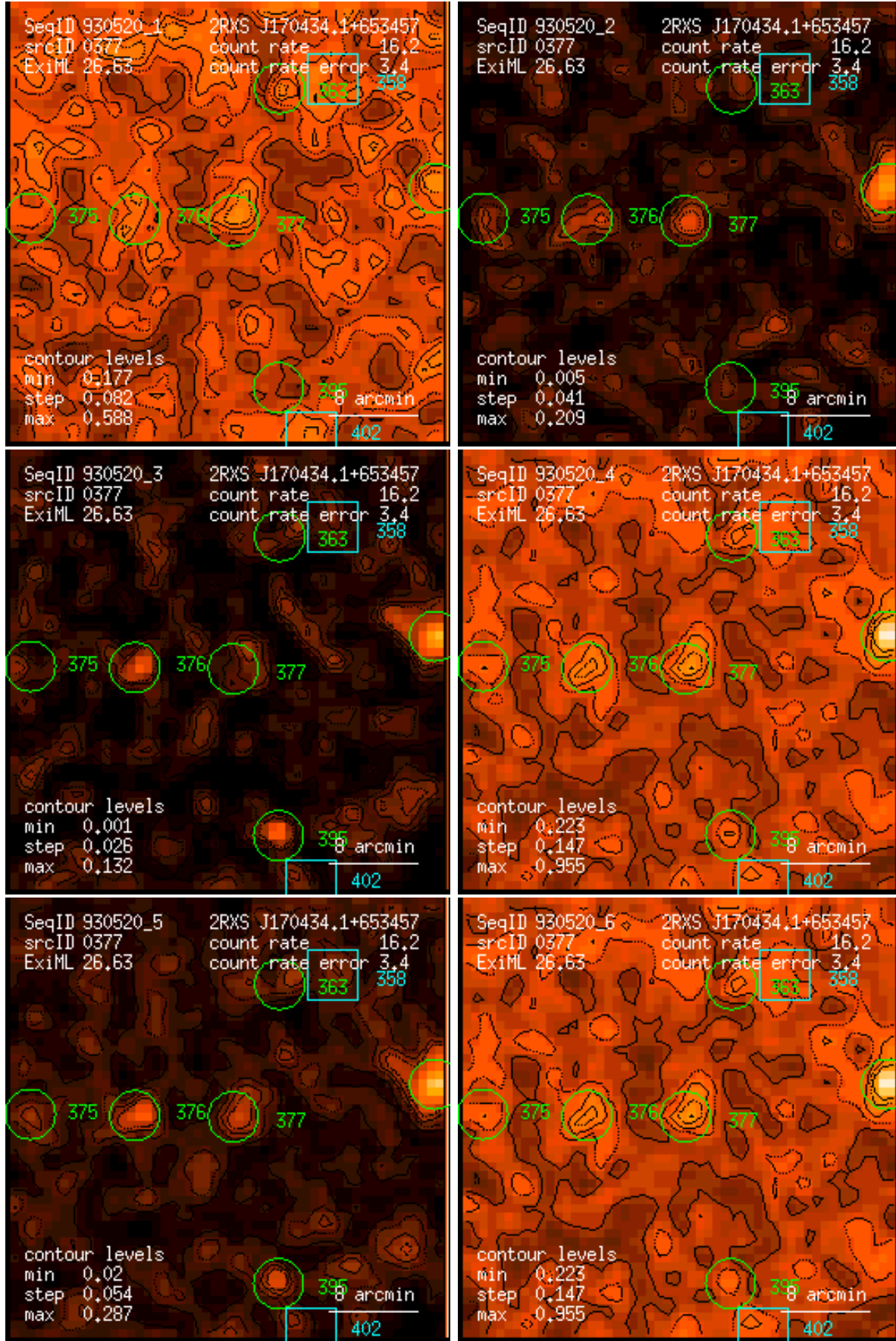
Figure 377: RASS 930520: detection 0377: band rate images, Gaussian filter: (1) PSPC channels 11 – 41, (2) 52 – 90, (3) 91 – 201, (4) 11 – 235, (5) 52 – 201, (6) 11 – 201. Broad band rates in counts/ks. Band rate contour levels in counts/ks/arcmin 2 .
