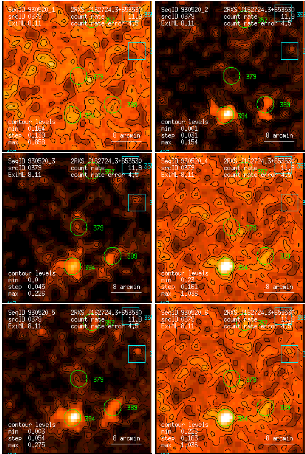
Figure 379: RASS 930520: detection 0379: band rate images, Gaussian filter: (1) PSPC channels 11 – 41, (2) 52 – 90, (3) 91 – 201, (4) 11 – 235, (5) 52 – 201, (6) 11 – 201. Broad band rates in counts/ks. Band rate contour levels in counts/ks/arcmin 2 .
