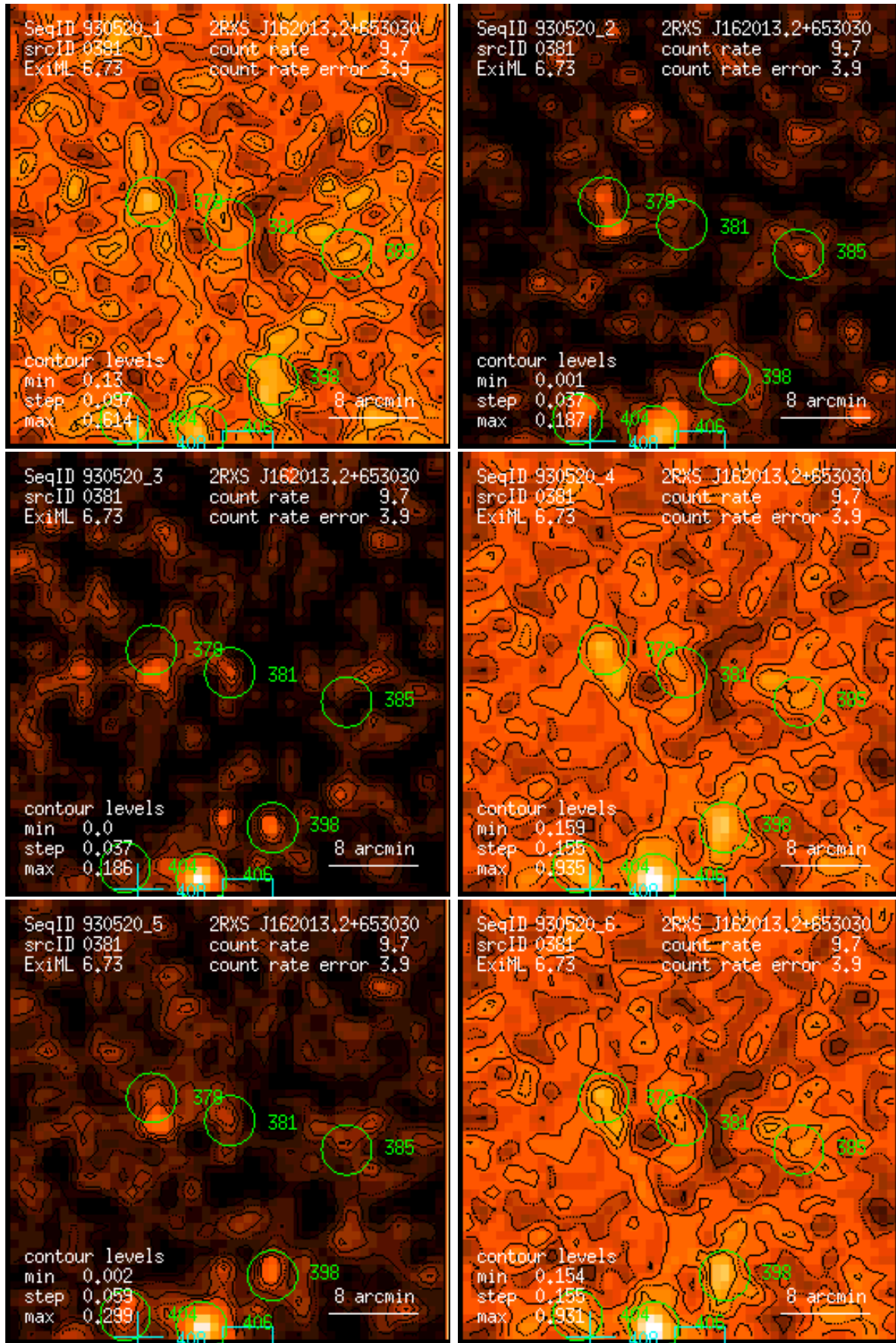
Figure 381: RASS 930520: detection 0381: band rate images, Gaussian filter: (1) PSPC channels 11 – 41, (2) 52 – 90, (3) 91 – 201, (4) 11 – 235, (5) 52 – 201, (6) 11 – 201. Broad band rates in counts/ks. Band rate contour levels in counts/ks/arcmin 2 .
