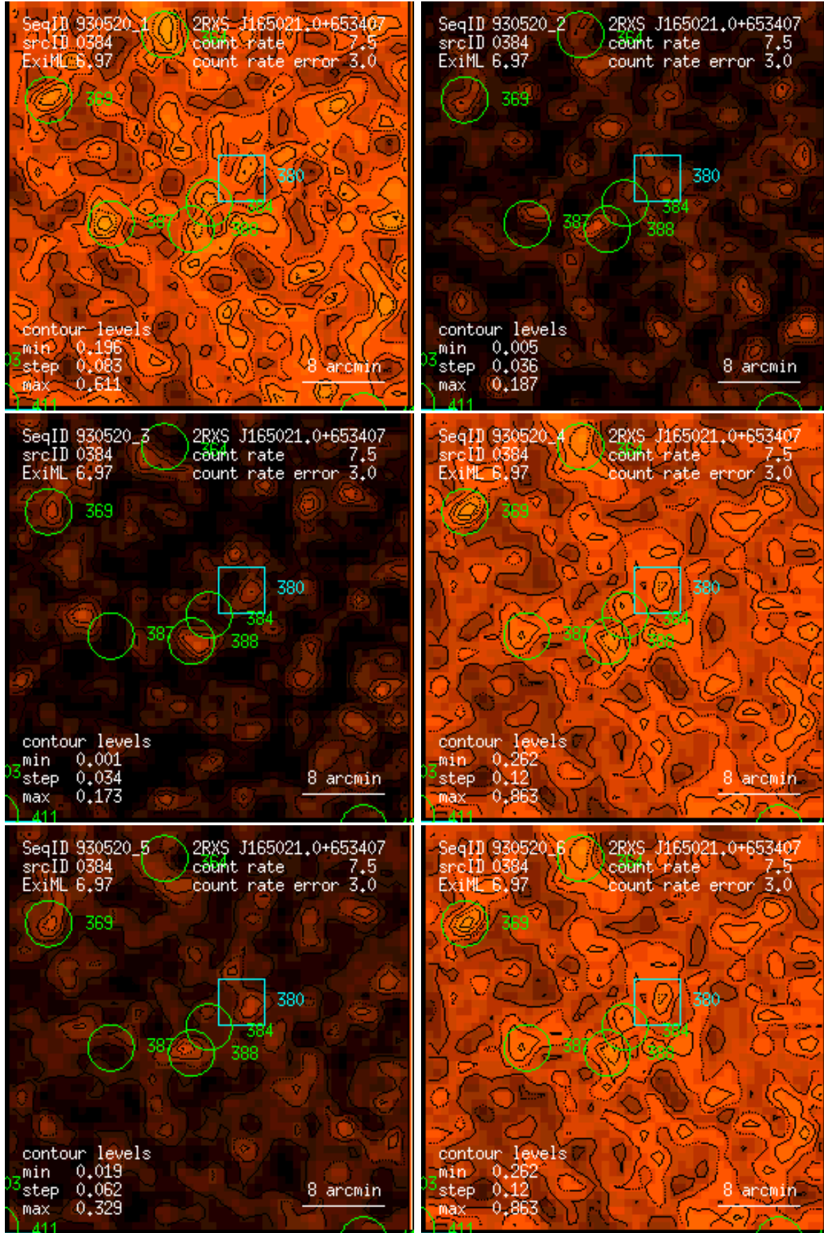
Figure 384: RASS 930520: detection 0384: band rate images, Gaussian filter: (1) PSPC channels 11 – 41, (2) 52 – 90, (3) 91 – 201, (4) 11 – 235, (5) 52 – 201, (6) 11 – 201. Broad band rates in counts/ks. Band rate contour levels in counts/ks/arcmin 2 .
