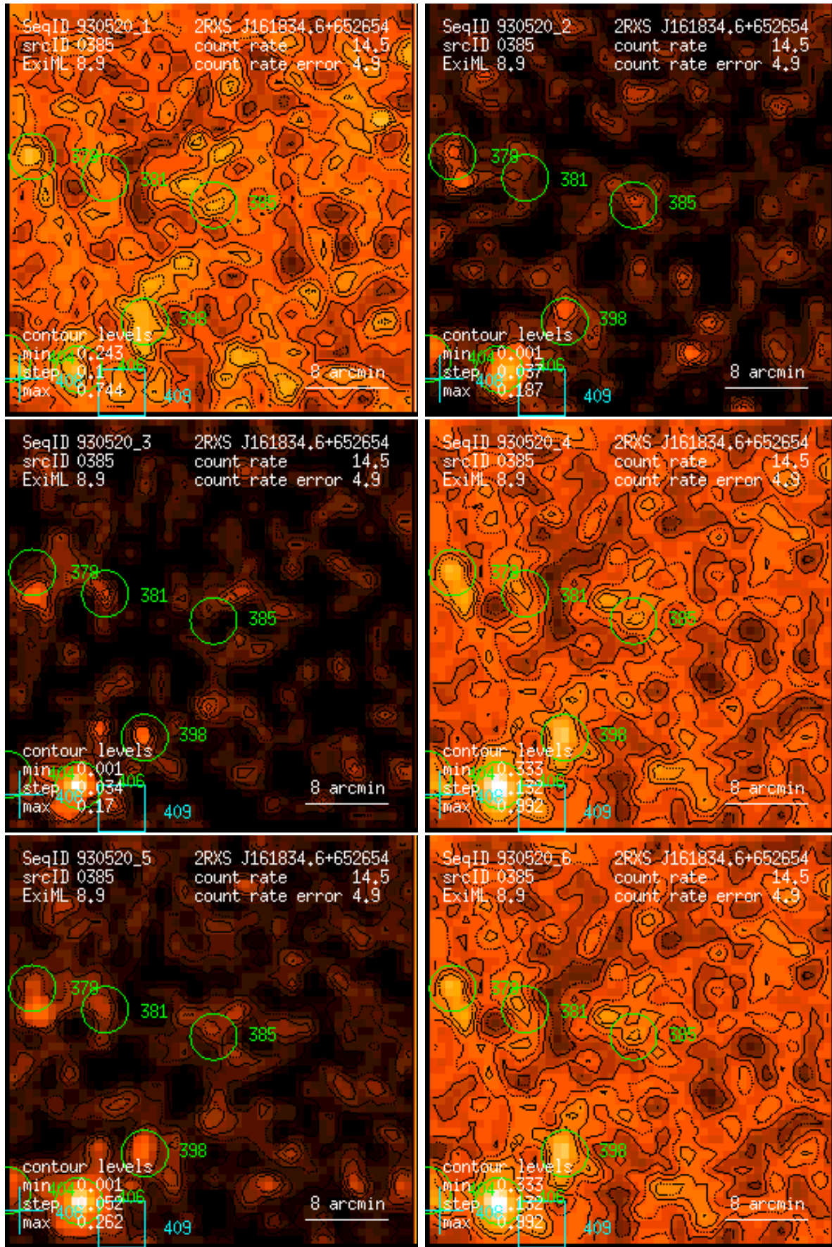
Figure 385: RASS 930520: detection 0385: band rate images, Gaussian filter: (1) PSPC channels 11 – 41, (2) 52 – 90, (3) 91 – 201, (4) 11 – 235, (5) 52 – 201, (6) 11 – 201. Broad band rates in counts/ks. Band rate contour levels in counts/ks/arcmin 2 .
