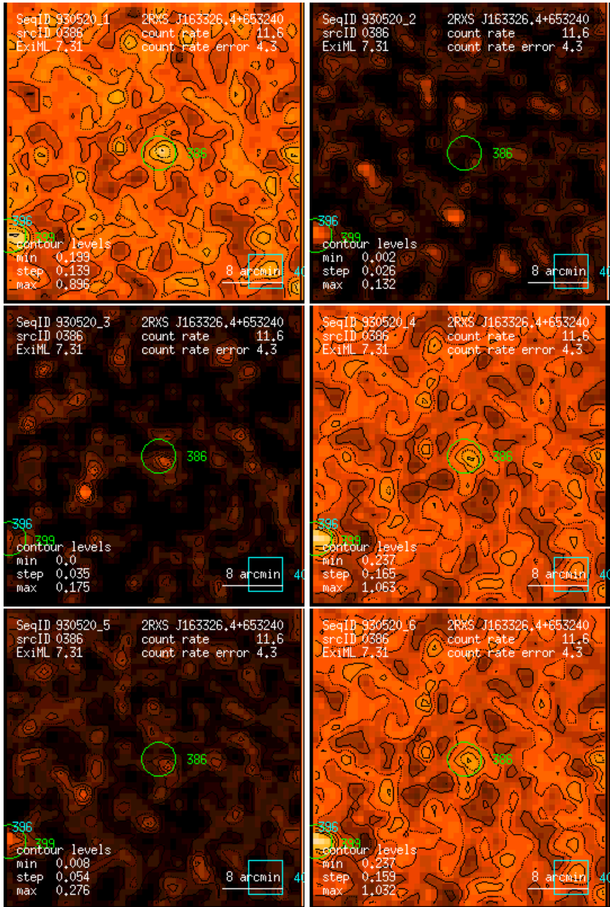
Figure 386: RASS 930520: detection 0386: band rate images, Gaussian filter: (1) PSPC channels 11 – 41, (2) 52 – 90, (3) 91 – 201, (4) 11 – 235, (5) 52 – 201, (6) 11 – 201. Broad band rates in counts/ks. Band rate contour levels in counts/ks/arcmin 2 .
