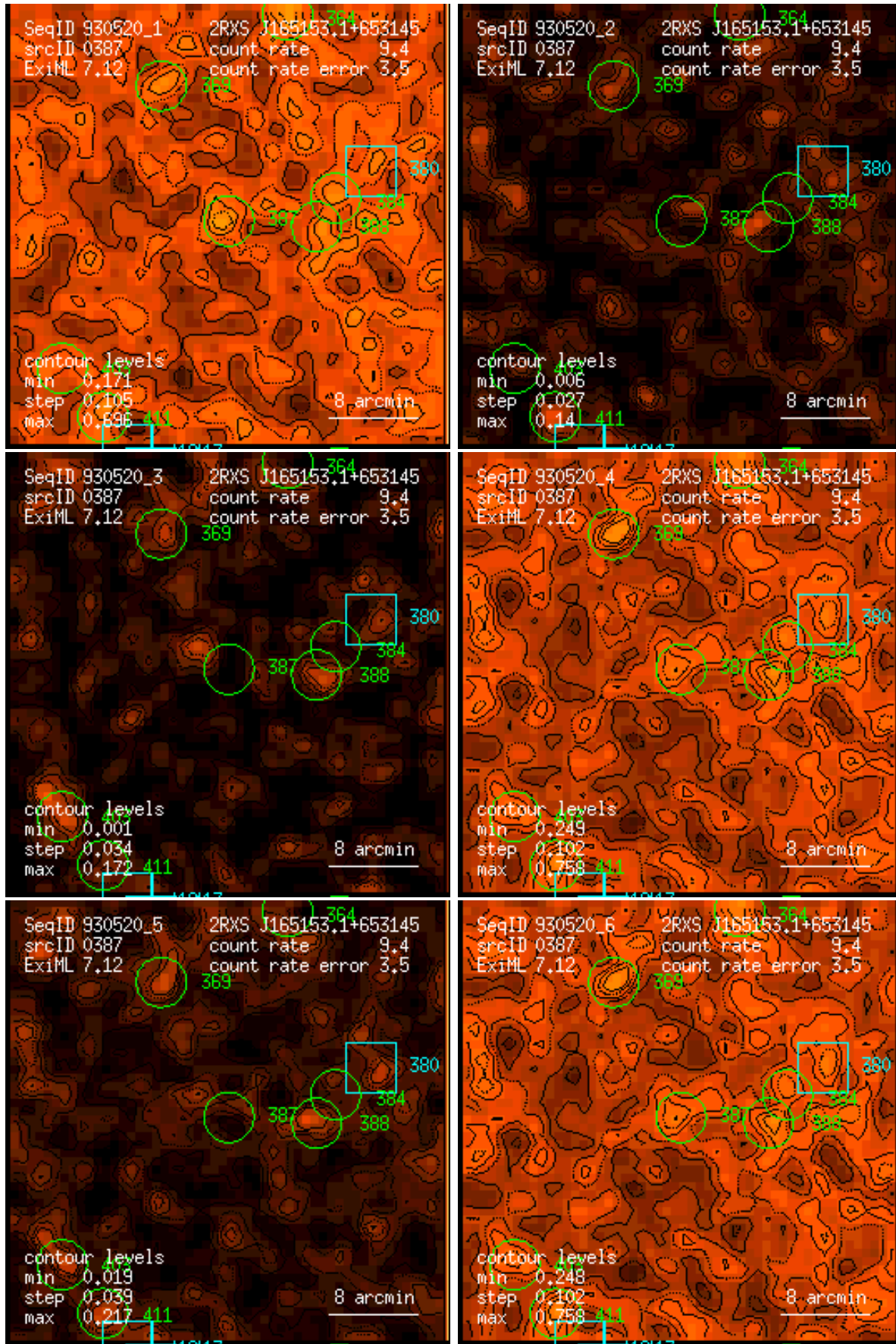
Figure 387: RASS 930520: detection 0387: band rate images, Gaussian filter: (1) PSPC channels 11 – 41, (2) 52 – 90, (3) 91 – 201, (4) 11 – 235, (5) 52 – 201, (6) 11 – 201. Broad band rates in counts/ks. Band rate contour levels in counts/ks/arcmin 2 .
