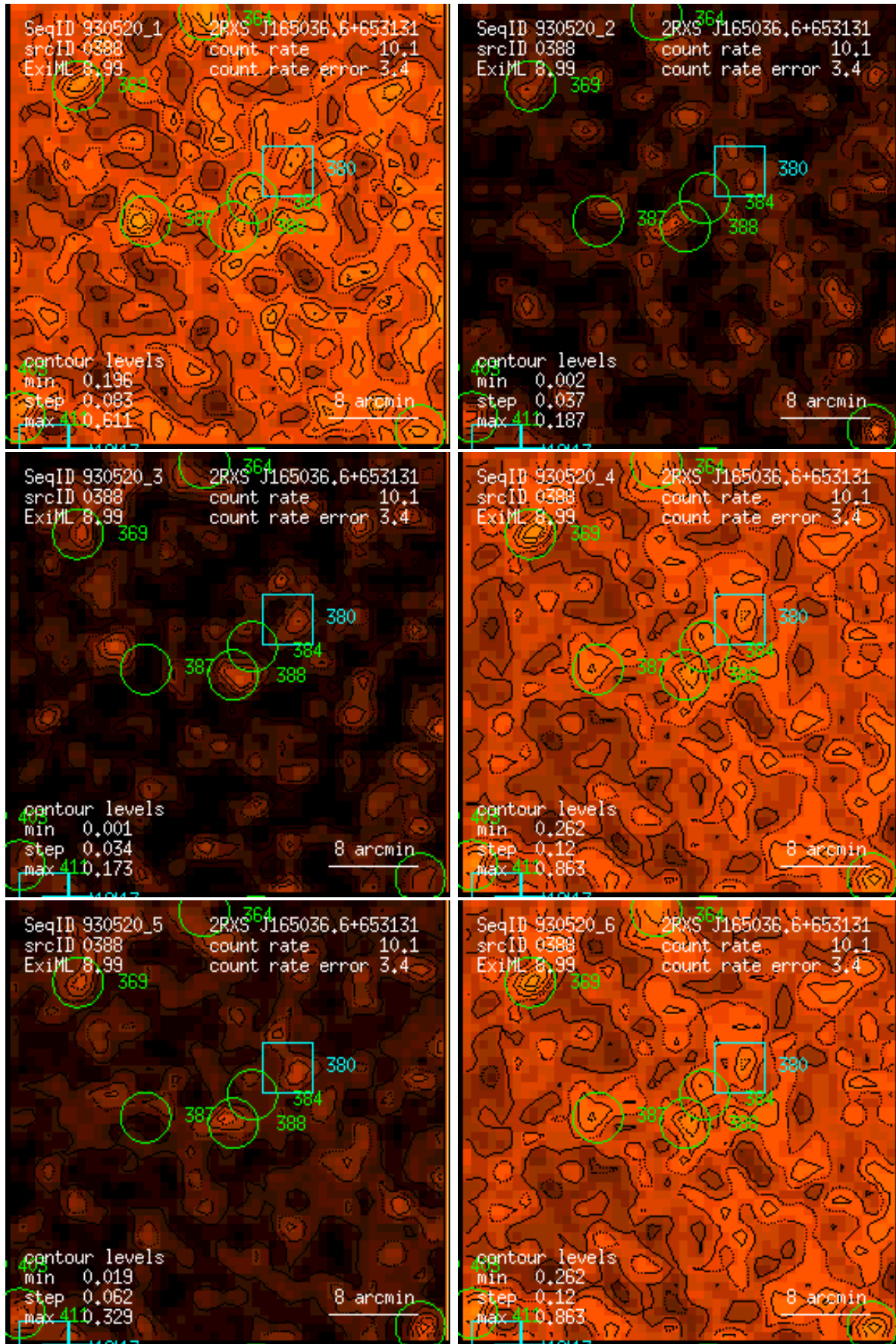
Figure 388: RASS 930520: detection 0388: band rate images, Gaussian filter: (1) PSPC channels 11 – 41, (2) 52 – 90, (3) 91 – 201, (4) 11 – 235, (5) 52 – 201, (6) 11 – 201. Broad band rates in counts/ks. Band rate contour levels in counts/ks/arcmin 2 .
