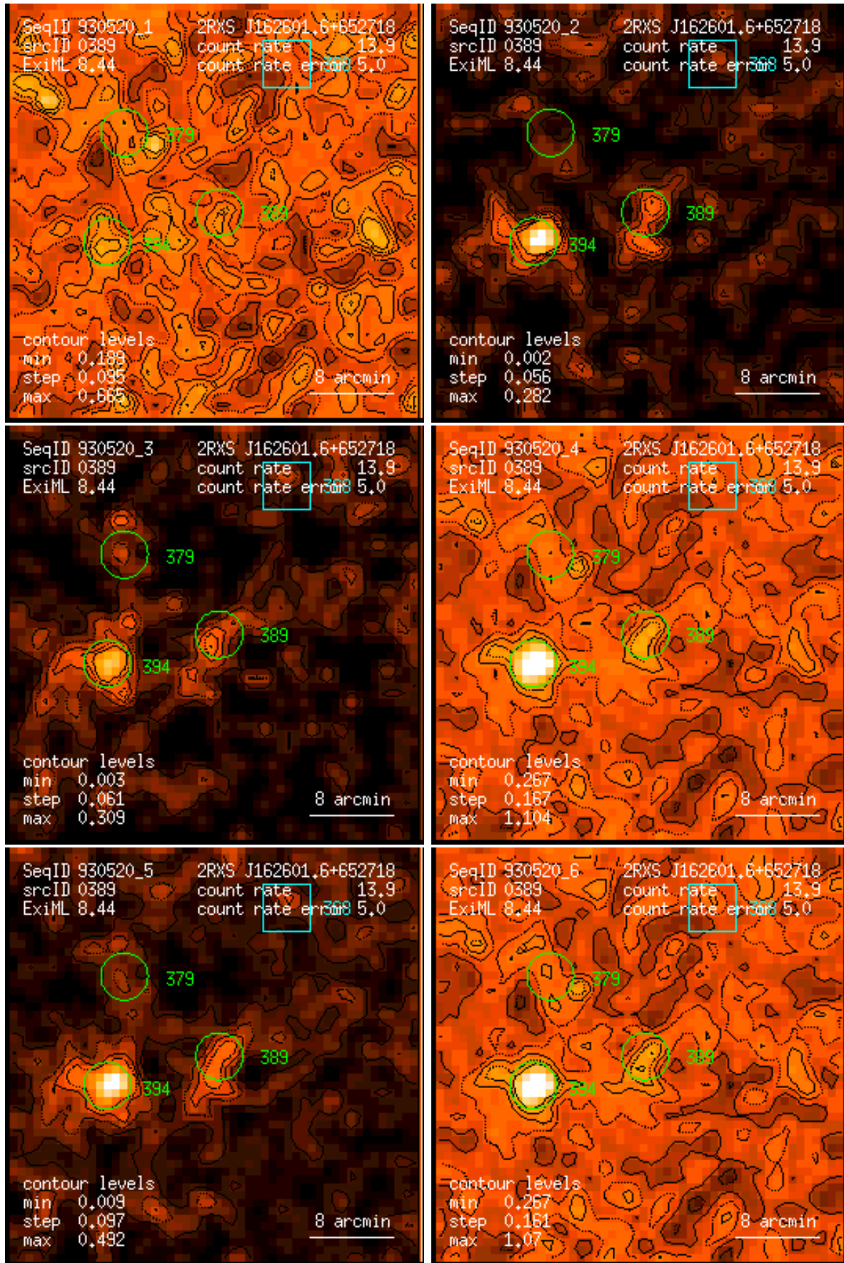
Figure 389: RASS 930520: detection 0389: band rate images, Gaussian filter: (1) PSPC channels 11 – 41, (2) 52 – 90, (3) 91 – 201, (4) 11 – 235, (5) 52 – 201, (6) 11 – 201. Broad band rates in counts/ks. Band rate contour levels in counts/ks/arcmin 2 .
