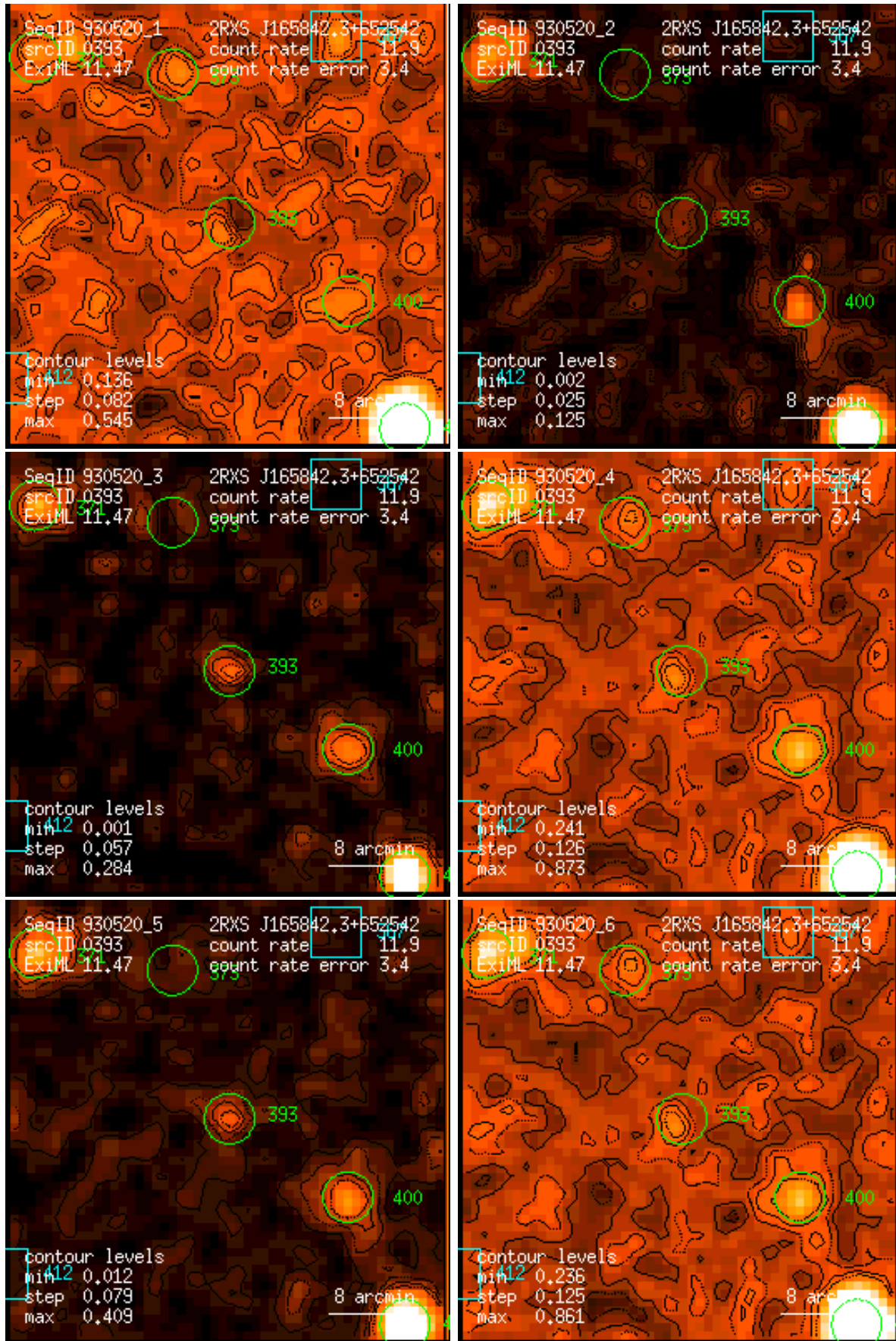
Figure 393: RASS 930520: detection 0393: band rate images, Gaussian filter: (1) PSPC channels 11 – 41, (2) 52 – 90, (3) 91 – 201, (4) 11 – 235, (5) 52 – 201, (6) 11 – 201. Broad band rates in counts/ks. Band rate contour levels in counts/ks/arcmin 2 .
