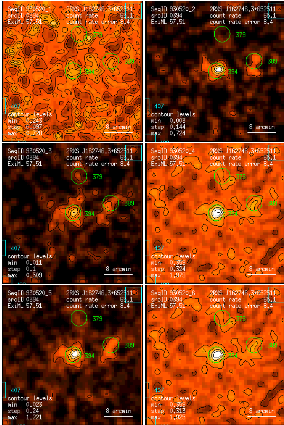
Figure 394: RASS 930520: detection 0394: band rate images, Gaussian filter: (1) PSPC channels 11 – 41, (2) 52 – 90, (3) 91 – 201, (4) 11 – 235, (5) 52 – 201, (6) 11 – 201. Broad band rates in counts/ks. Band rate contour levels in counts/ks/arcmin 2 .
