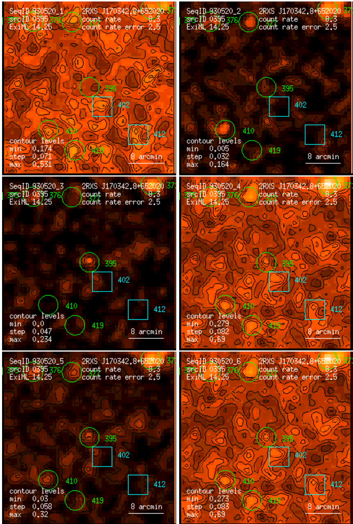
Figure 395: RASS 930520: detection 0395: band rate images, Gaussian filter: (1) PSPC channels 11 – 41, (2) 52 – 90, (3) 91 – 201, (4) 11 – 235, (5) 52 – 201, (6) 11 – 201. Broad band rates in counts/ks. Band rate contour levels in counts/ks/arcmin 2 .
