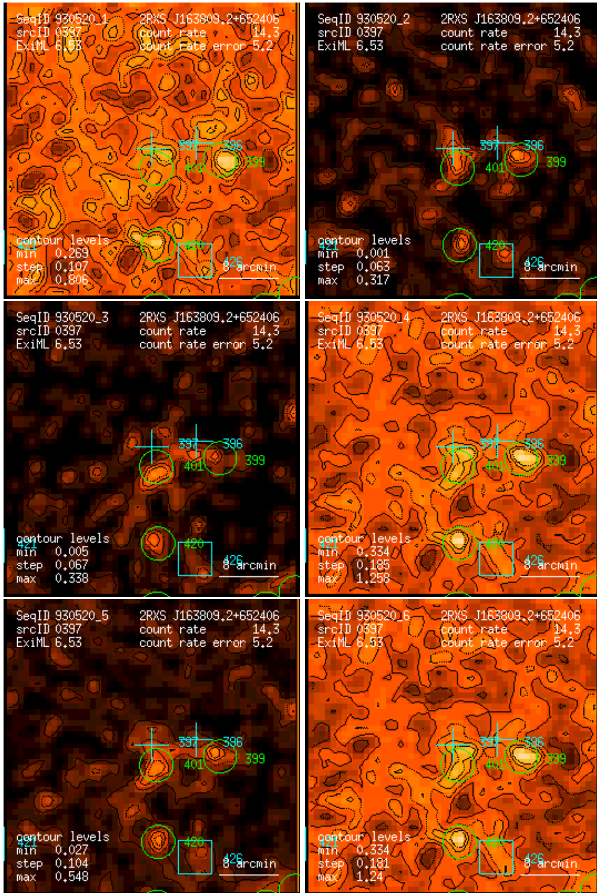
Figure 397: RASS 930520: detection 0397: band rate images, Gaussian filter: (1) PSPC channels 11 – 41, (2) 52 – 90, (3) 91 – 201, (4) 11 – 235, (5) 52 – 201, (6) 11 – 201. Broad band rates in counts/ks. Band rate contour levels in counts/ks/arcmin 2 .
