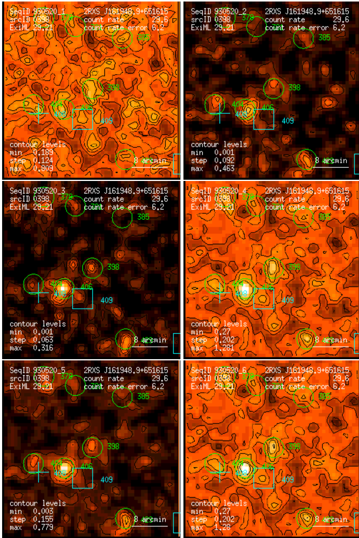
Figure 398: RASS 930520: detection 0398: band rate images, Gaussian filter: (1) PSPC channels 11 – 41, (2) 52 – 90, (3) 91 – 201, (4) 11 – 235, (5) 52 – 201, (6) 11 – 201. Broad band rates in counts/ks. Band rate contour levels in counts/ks/arcmin 2 .
