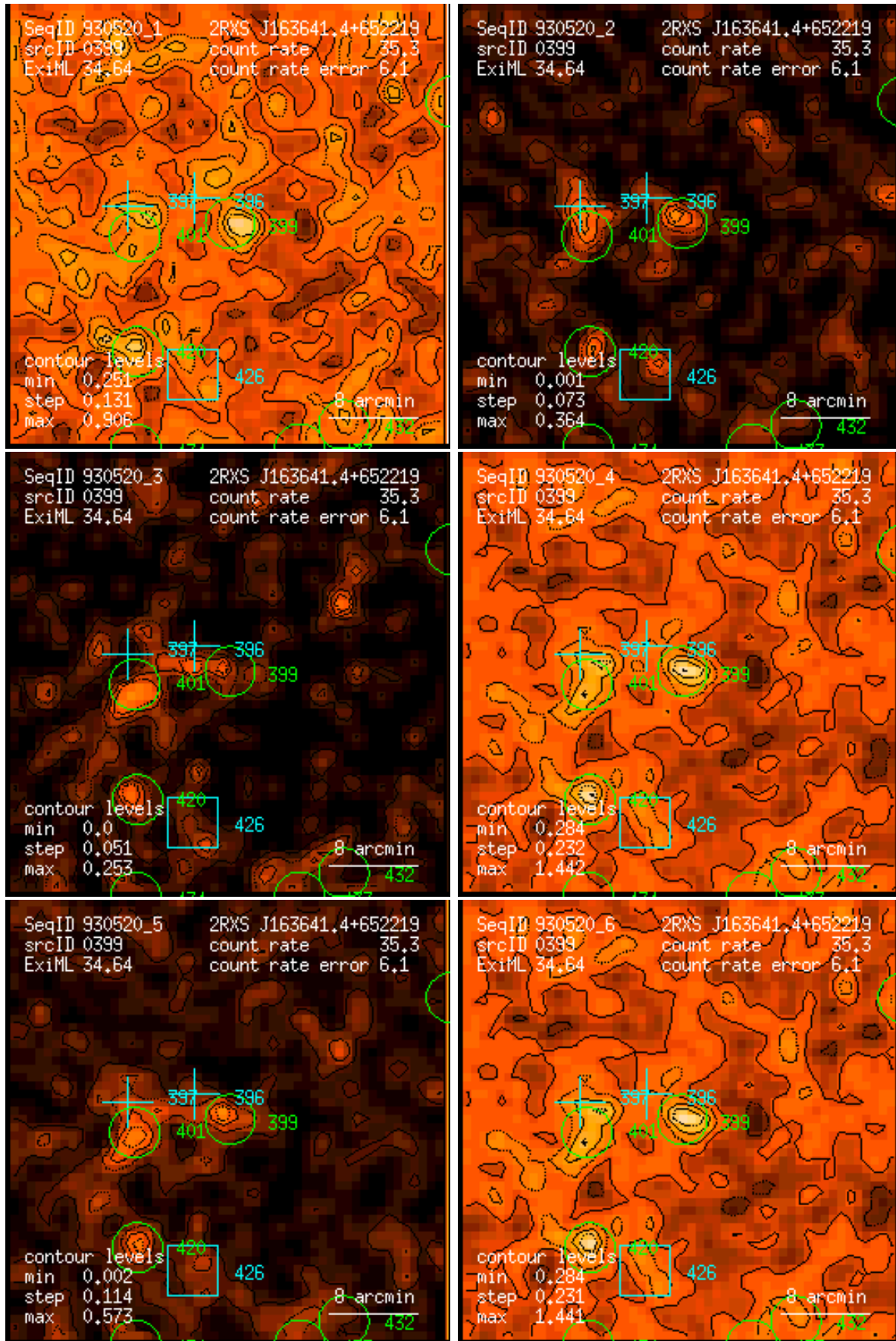
Figure 399: RASS 930520: detection 0399: band rate images, Gaussian filter: (1) PSPC channels 11 – 41, (2) 52 – 90, (3) 91 – 201, (4) 11 – 235, (5) 52 – 201, (6) 11 – 201. Broad band rates in counts/ks. Band rate contour levels in counts/ks/arcmin 2 .
