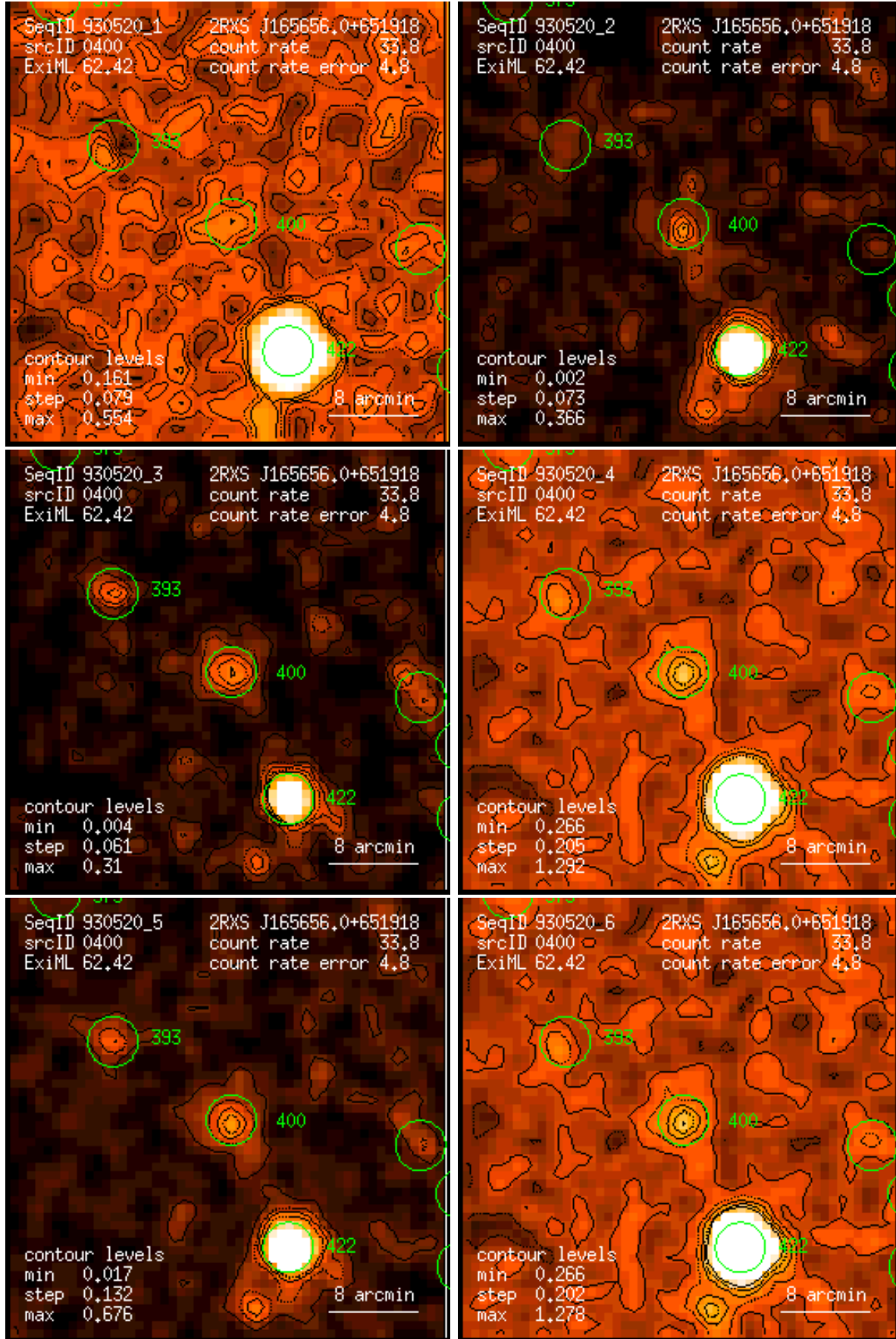
Figure 400: RASS 930520: detection 0400: band rate images, Gaussian filter: (1) PSPC channels 11 – 41, (2) 52 – 90, (3) 91 – 201, (4) 11 – 235, (5) 52 – 201, (6) 11 – 201. Broad band rates in counts/ks. Band rate contour levels in counts/ks/arcmin 2 .
