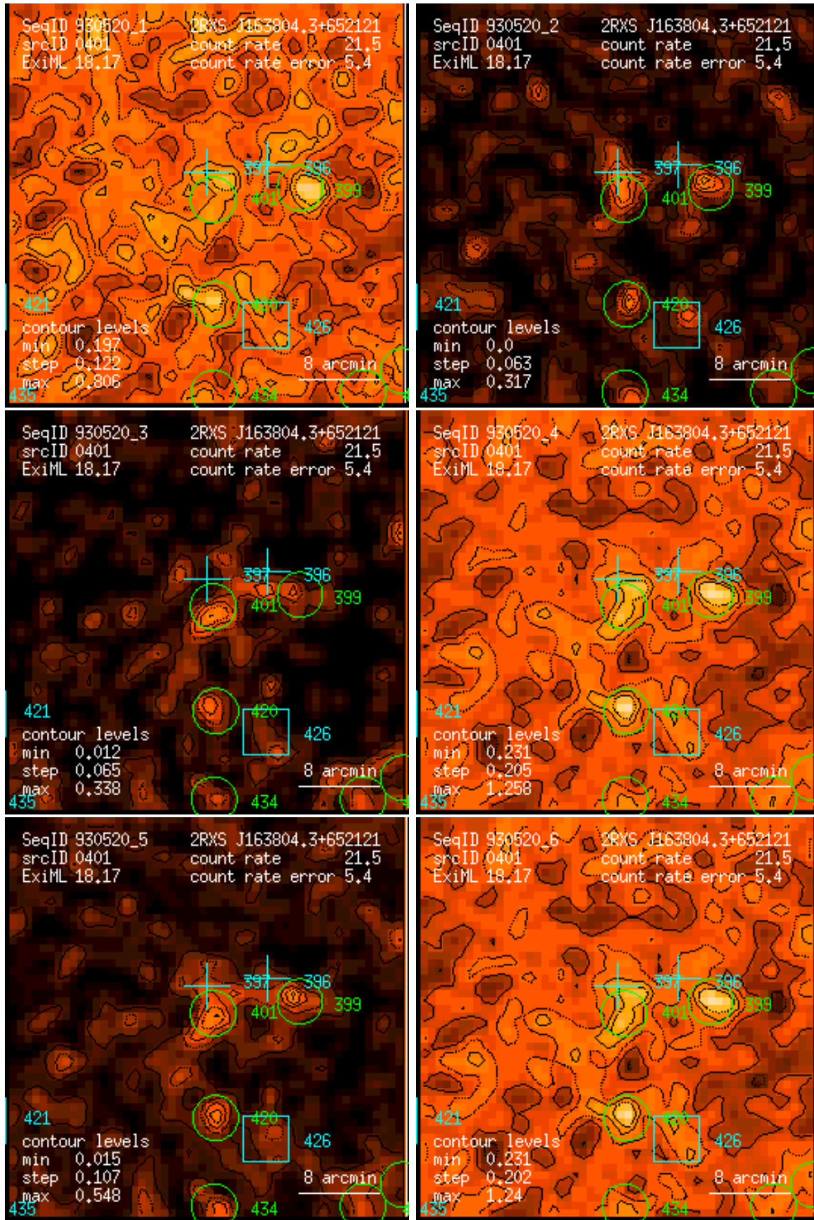
Figure 401: RASS 930520: detection 0401: band rate images, Gaussian filter: (1) PSPC channels 11 – 41, (2) 52 – 90, (3) 91 – 201, (4) 11 – 235, (5) 52 – 201, (6) 11 – 201. Broad band rates in counts/ks. Band rate contour levels in counts/ks/arcmin 2 .
