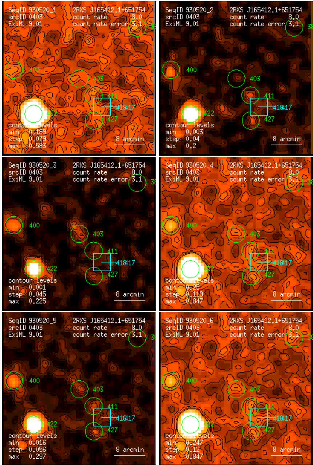
Figure 403: RASS 930520: detection 0403: band rate images, Gaussian filter: (1) PSPC channels 11 – 41, (2) 52 – 90, (3) 91 – 201, (4) 11 – 235, (5) 52 – 201, (6) 11 – 201. Broad band rates in counts/ks. Band rate contour levels in counts/ks/arcmin 2 .
