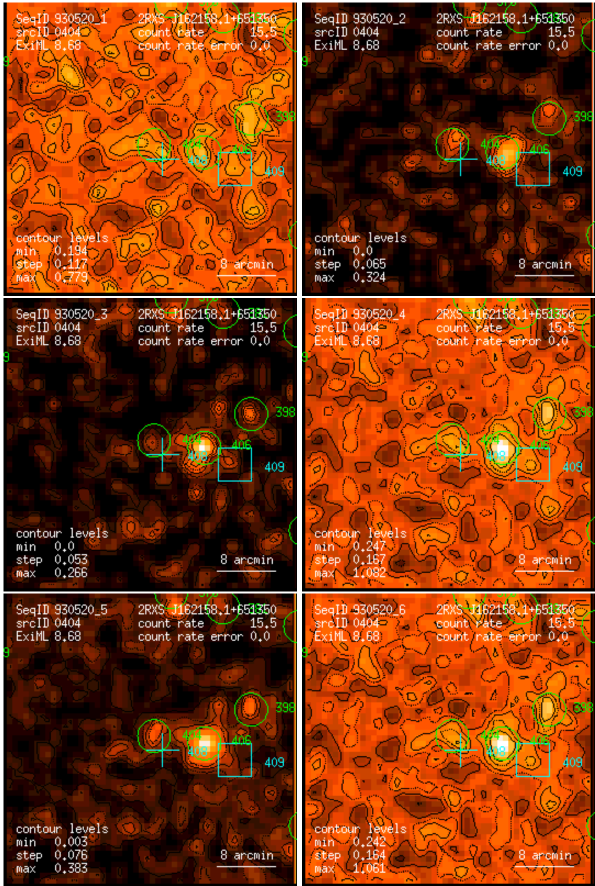
Figure 404: RASS 930520: detection 0404: band rate images, Gaussian filter: (1) PSPC channels 11 – 41, (2) 52 – 90, (3) 91 – 201, (4) 11 – 235, (5) 52 – 201, (6) 11 – 201. Broad band rates in counts/ks. Band rate contour levels in counts/ks/arcmin 2 .
