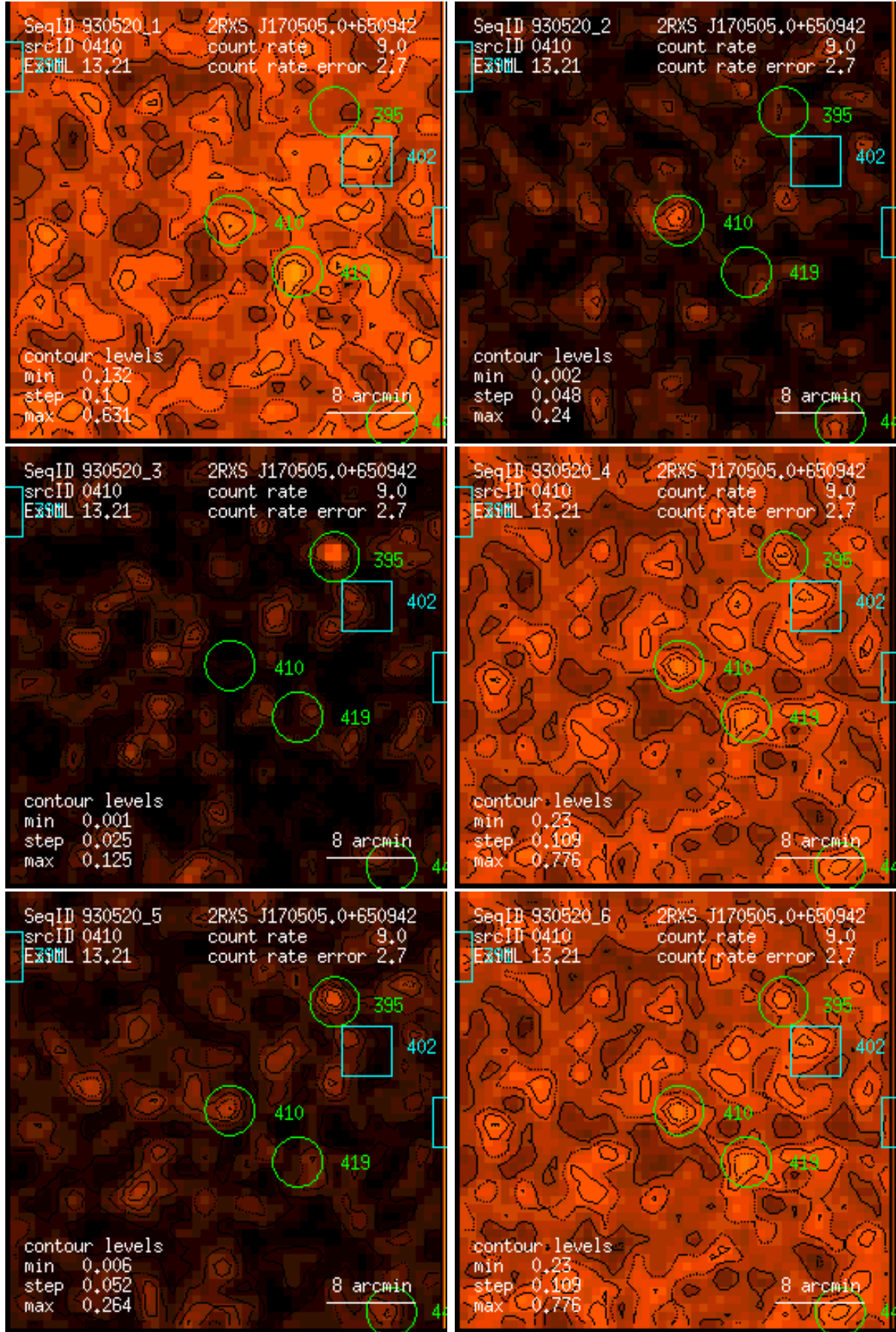
Figure 410: RASS 930520: detection 0410: band rate images, Gaussian filter: (1) PSPC channels 11 – 41, (2) 52 – 90, (3) 91 – 201, (4) 11 – 235, (5) 52 – 201, (6) 11 – 201. Broad band rates in counts/ks. Band rate contour levels in counts/ks/arcmin 2 .
