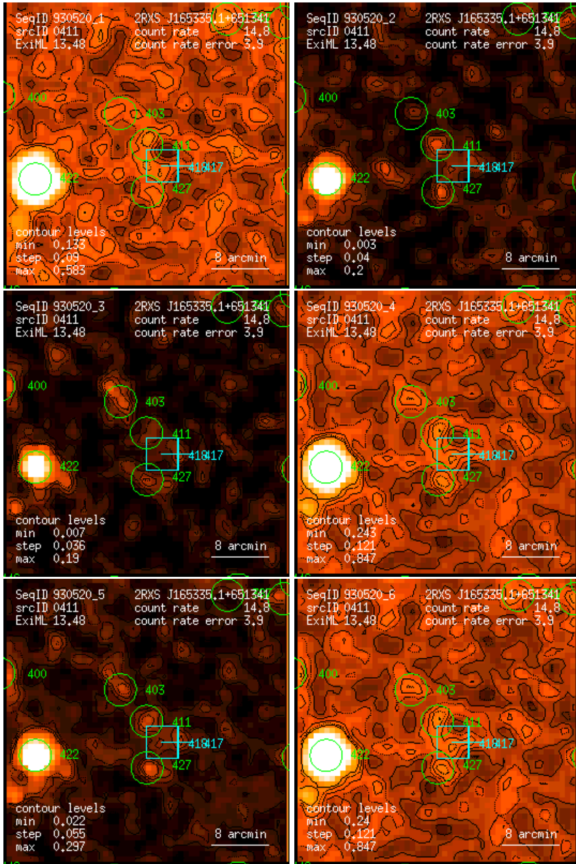
Figure 411: RASS 930520: detection 0411: band rate images, Gaussian filter: (1) PSPC channels 11 – 41, (2) 52 – 90, (3) 91 – 201, (4) 11 – 235, (5) 52 – 201, (6) 11 – 201. Broad band rates in counts/ks. Band rate contour levels in counts/ks/arcmin 2 .
