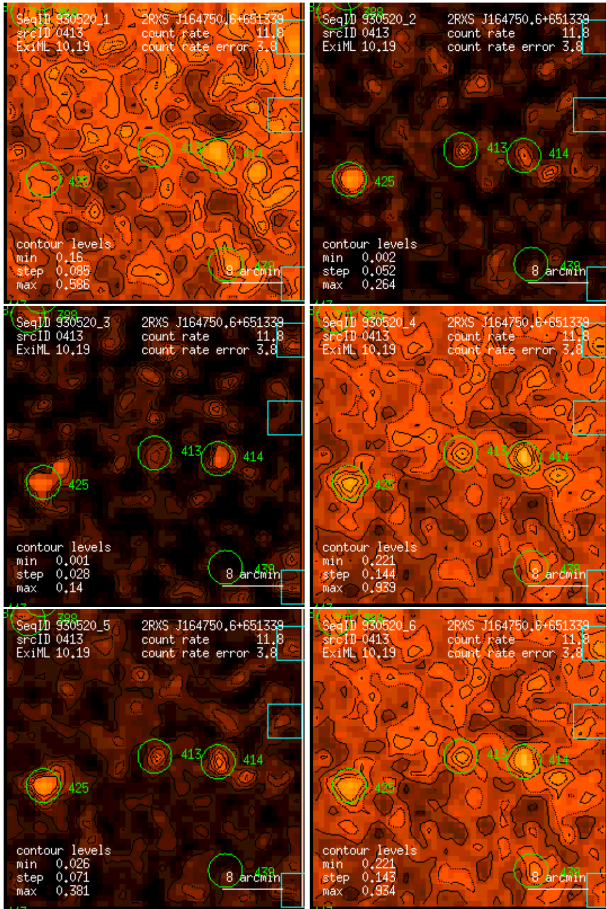
Figure 413: RASS 930520: detection 0413: band rate images, Gaussian filter: (1) PSPC channels 11 – 41, (2) 52 – 90, (3) 91 – 201, (4) 11 – 235, (5) 52 – 201, (6) 11 – 201. Broad band rates in counts/ks. Band rate contour levels in counts/ks/arcmin 2 .
