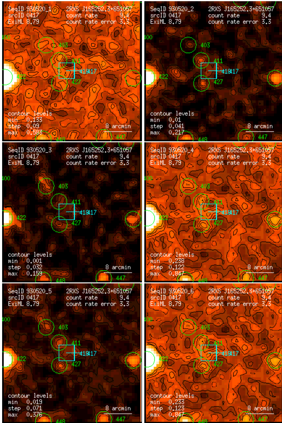
Figure 417: RASS 930520: detection 0417: band rate images, Gaussian filter: (1) PSPC channels 11 – 41, (2) 52 – 90, (3) 91 – 201, (4) 11 – 235, (5) 52 – 201, (6) 11 – 201. Broad band rates in counts/ks. Band rate contour levels in counts/ks/arcmin 2 .
