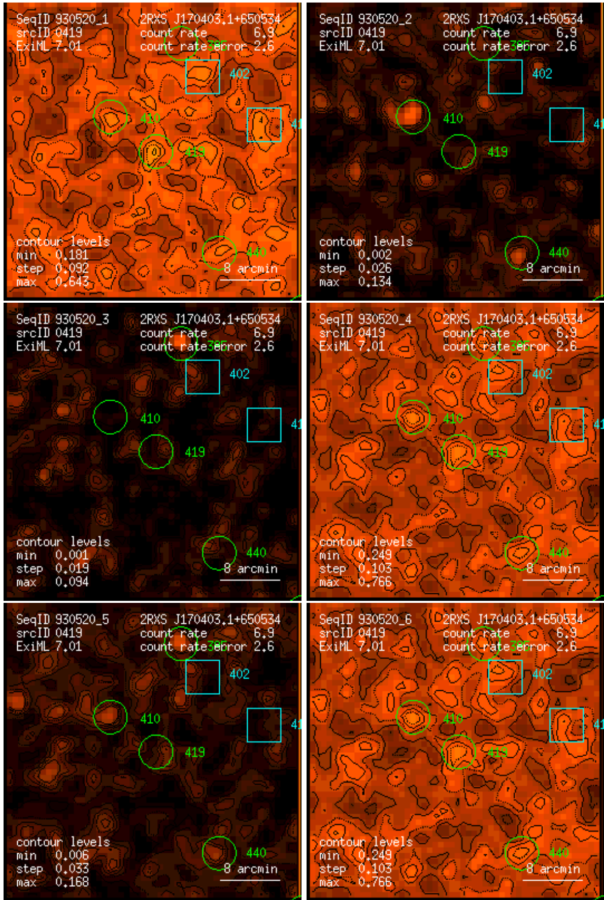
Figure 419: RASS 930520: detection 0419: band rate images, Gaussian filter: (1) PSPC channels 11 – 41, (2) 52 – 90, (3) 91 – 201, (4) 11 – 235, (5) 52 – 201, (6) 11 – 201. Broad band rates in counts/ks. Band rate contour levels in counts/ks/arcmin 2 .
