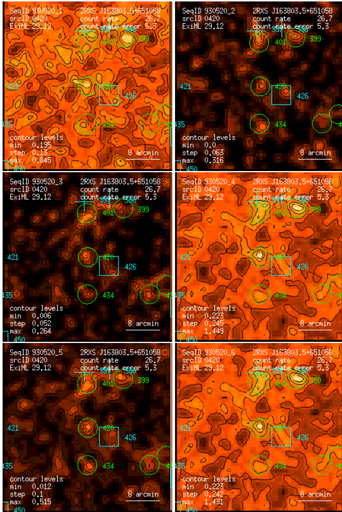
Figure 420: RASS 930520: detection 0420: band rate images, Gaussian filter: (1) PSPC channels 11 – 41, (2) 52 – 90, (3) 91 – 201, (4) 11 – 235, (5) 52 – 201, (6) 11 – 201. Broad band rates in counts/ks. Band rate contour levels in counts/ks/arcmin 2 .
