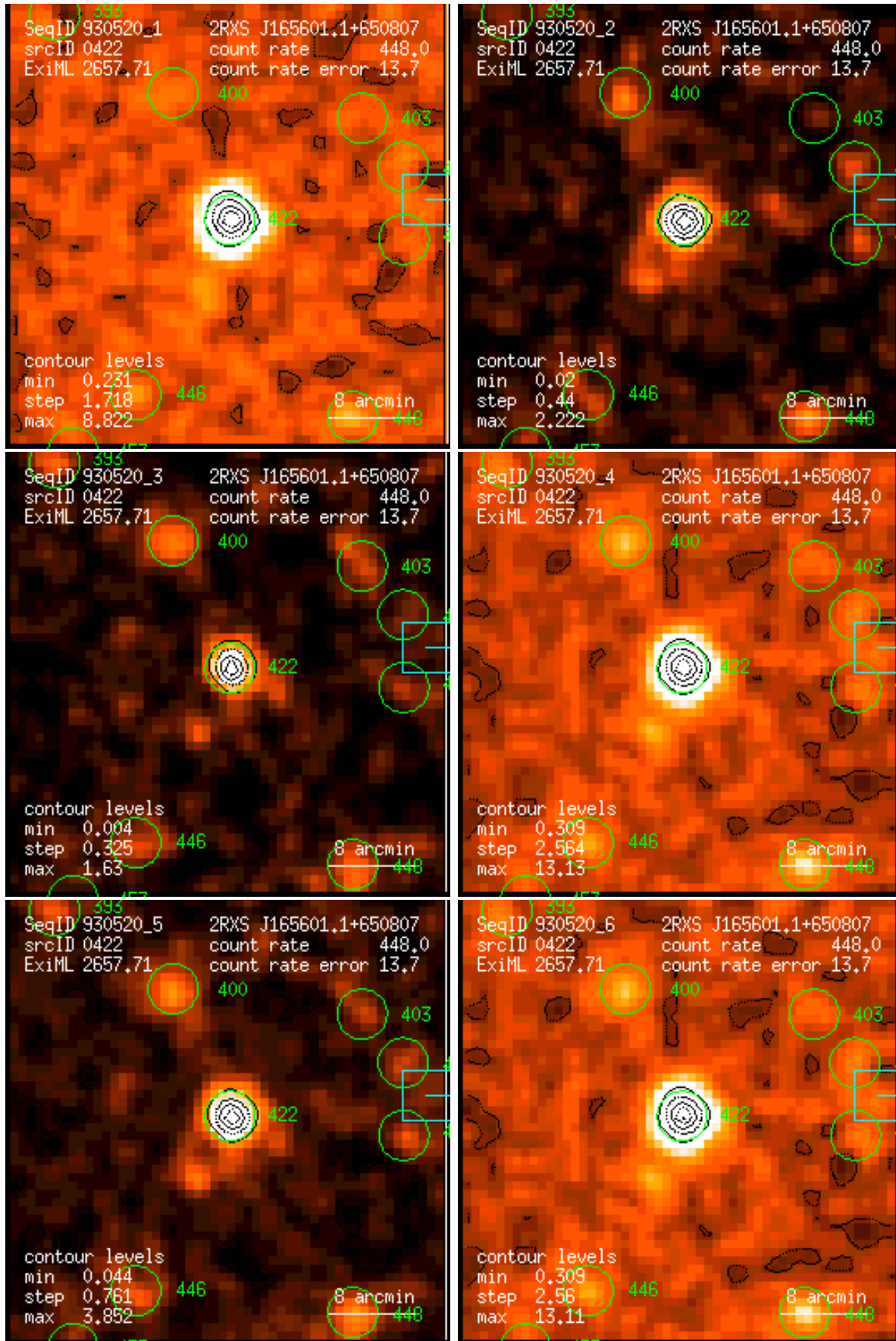
Figure 422: RASS 930520: detection 0422: band rate images, Gaussian filter: (1) PSPC channels 11 – 41, (2) 52 – 90, (3) 91 – 201, (4) 11 – 235, (5) 52 – 201, (6) 11 – 201. Broad band rates in counts/ks. Band rate contour levels in counts/ks/arcmin 2 .
