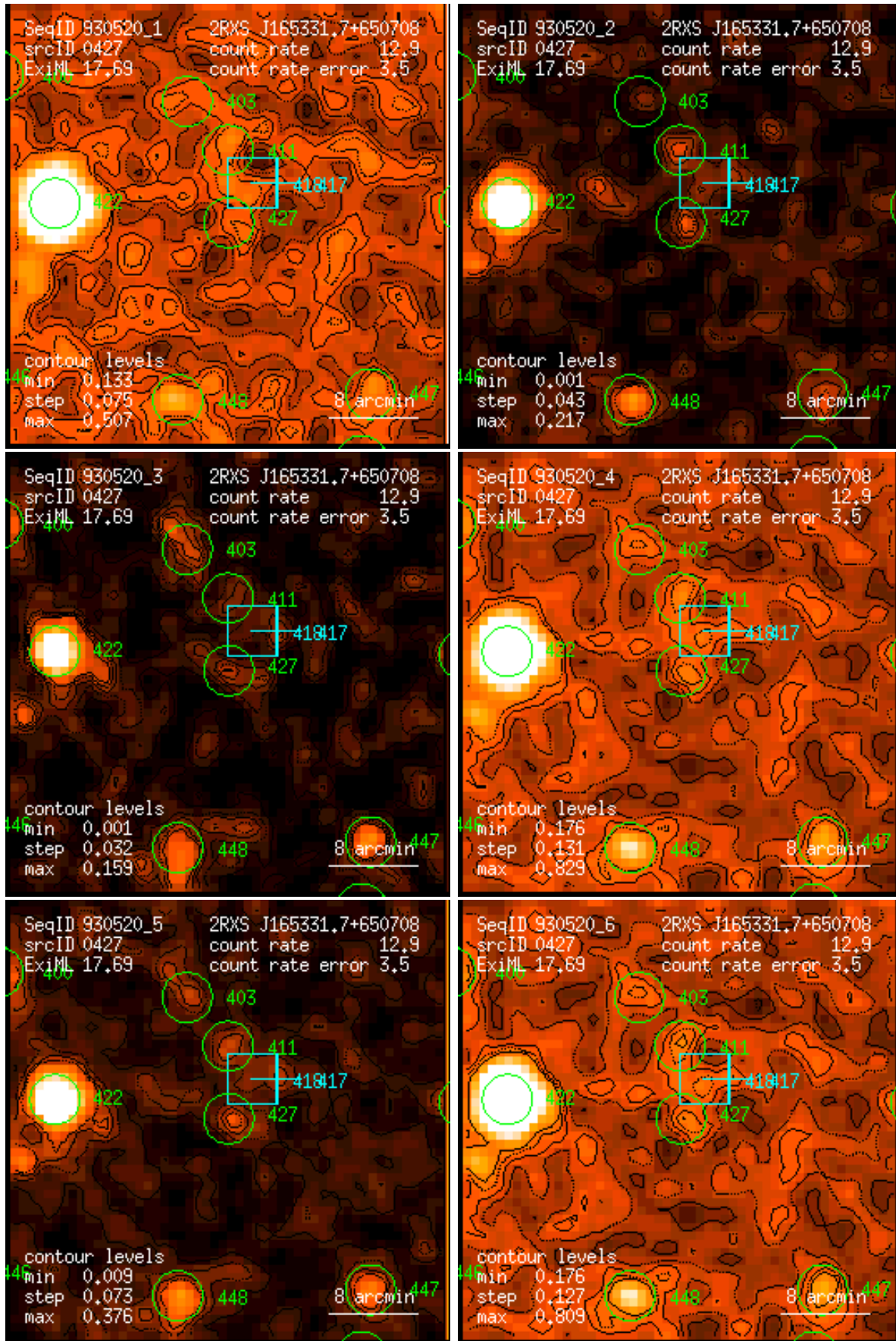
Figure 427: RASS 930520: detection 0427: band rate images, Gaussian filter: (1) PSPC channels 11 – 41, (2) 52 – 90, (3) 91 – 201, (4) 11 – 235, (5) 52 – 201, (6) 11 – 201. Broad band rates in counts/ks. Band rate contour levels in counts/ks/arcmin 2 .
