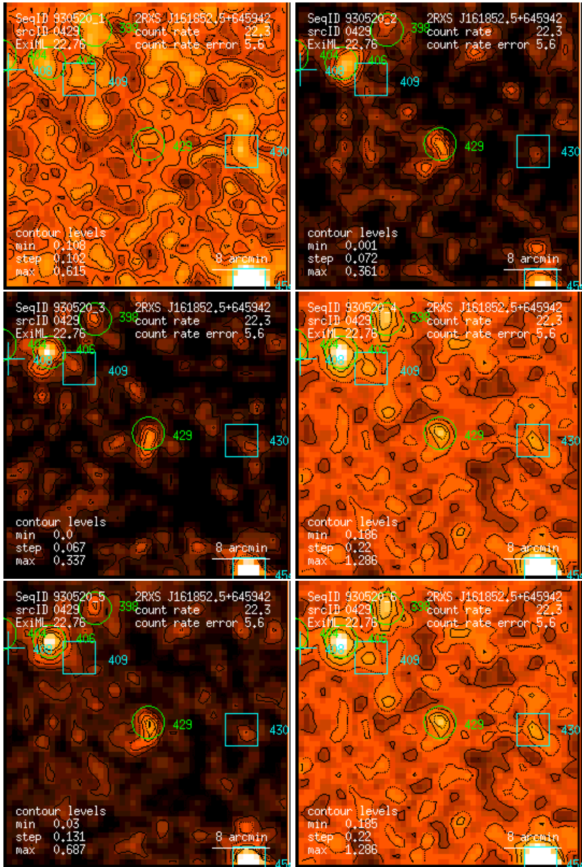
Figure 429: RASS 930520: detection 0429: band rate images, Gaussian filter: (1) PSPC channels 11 – 41, (2) 52 – 90, (3) 91 – 201, (4) 11 – 235, (5) 52 – 201, (6) 11 – 201. Broad band rates in counts/ks. Band rate contour levels in counts/ks/arcmin 2 .
