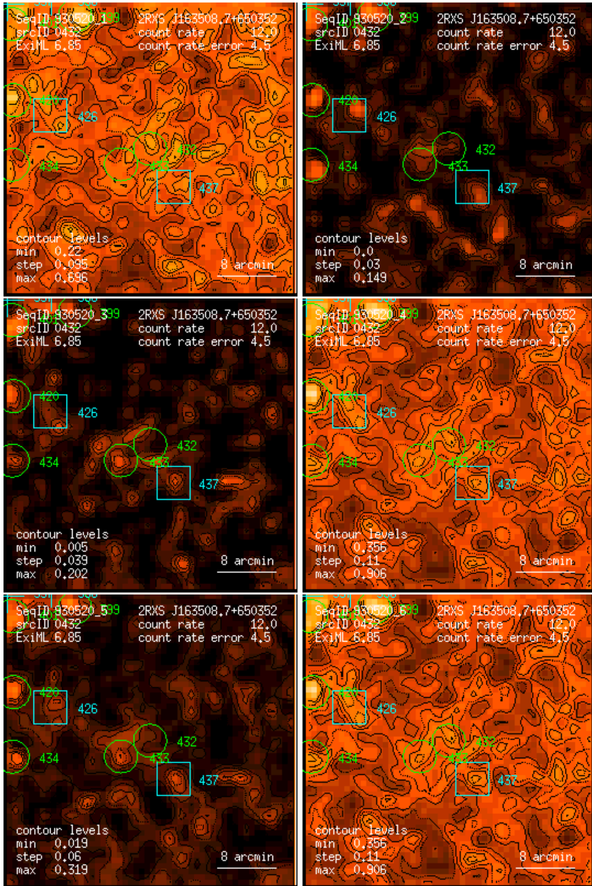
Figure 432: RASS 930520: detection 0432: band rate images, Gaussian filter: (1) PSPC channels 11 – 41, (2) 52 – 90, (3) 91 – 201, (4) 11 – 235, (5) 52 – 201, (6) 11 – 201. Broad band rates in counts/ks. Band rate contour levels in counts/ks/arcmin 2 .
