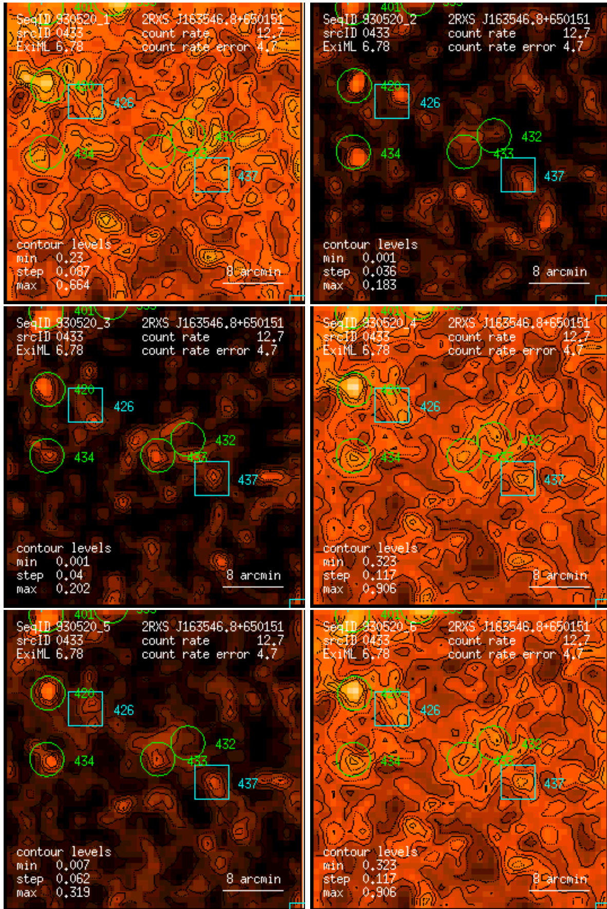
Figure 433: RASS 930520: detection 0433: band rate images, Gaussian filter: (1) PSPC channels 11 – 41, (2) 52 – 90, (3) 91 – 201, (4) 11 – 235, (5) 52 – 201, (6) 11 – 201. Broad band rates in counts/ks. Band rate contour levels in counts/ks/arcmin 2 .
