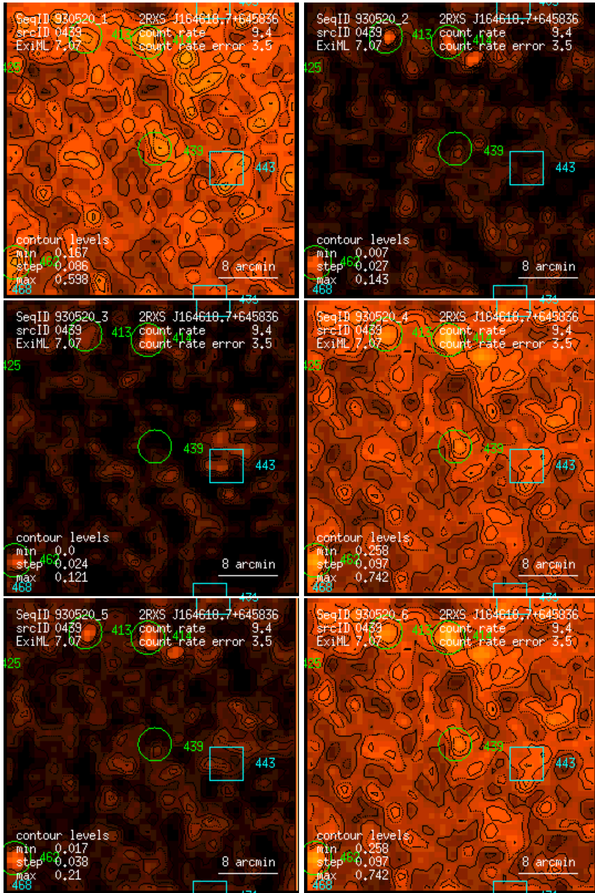
Figure 439: RASS 930520: detection 0439: band rate images, Gaussian filter: (1) PSPC channels 11 – 41, (2) 52 – 90, (3) 91 – 201, (4) 11 – 235, (5) 52 – 201, (6) 11 – 201. Broad band rates in counts/ks. Band rate contour levels in counts/ks/arcmin 2 .
