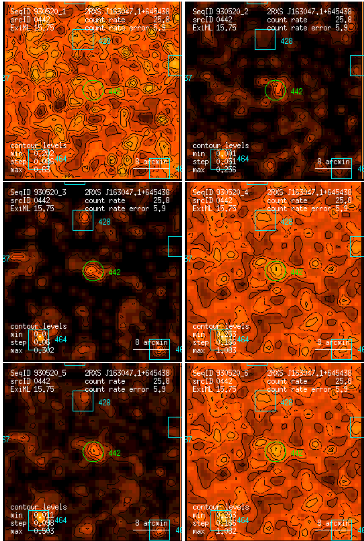
Figure 442: RASS 930520: detection 0442: band rate images, Gaussian filter: (1) PSPC channels 11 – 41, (2) 52 – 90, (3) 91 – 201, (4) 11 – 235, (5) 52 – 201, (6) 11 – 201. Broad band rates in counts/ks. Band rate contour levels in counts/ks/arcmin 2 .
