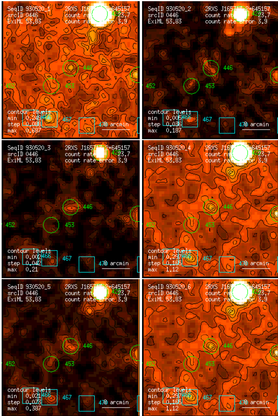
Figure 446: RASS 930520: detection 0446: band rate images, Gaussian filter: (1) PSPC channels 11 – 41, (2) 52 – 90, (3) 91 – 201, (4) 11 – 235, (5) 52 – 201, (6) 11 – 201. Broad band rates in counts/ks. Band rate contour levels in counts/ks/arcmin 2 .
