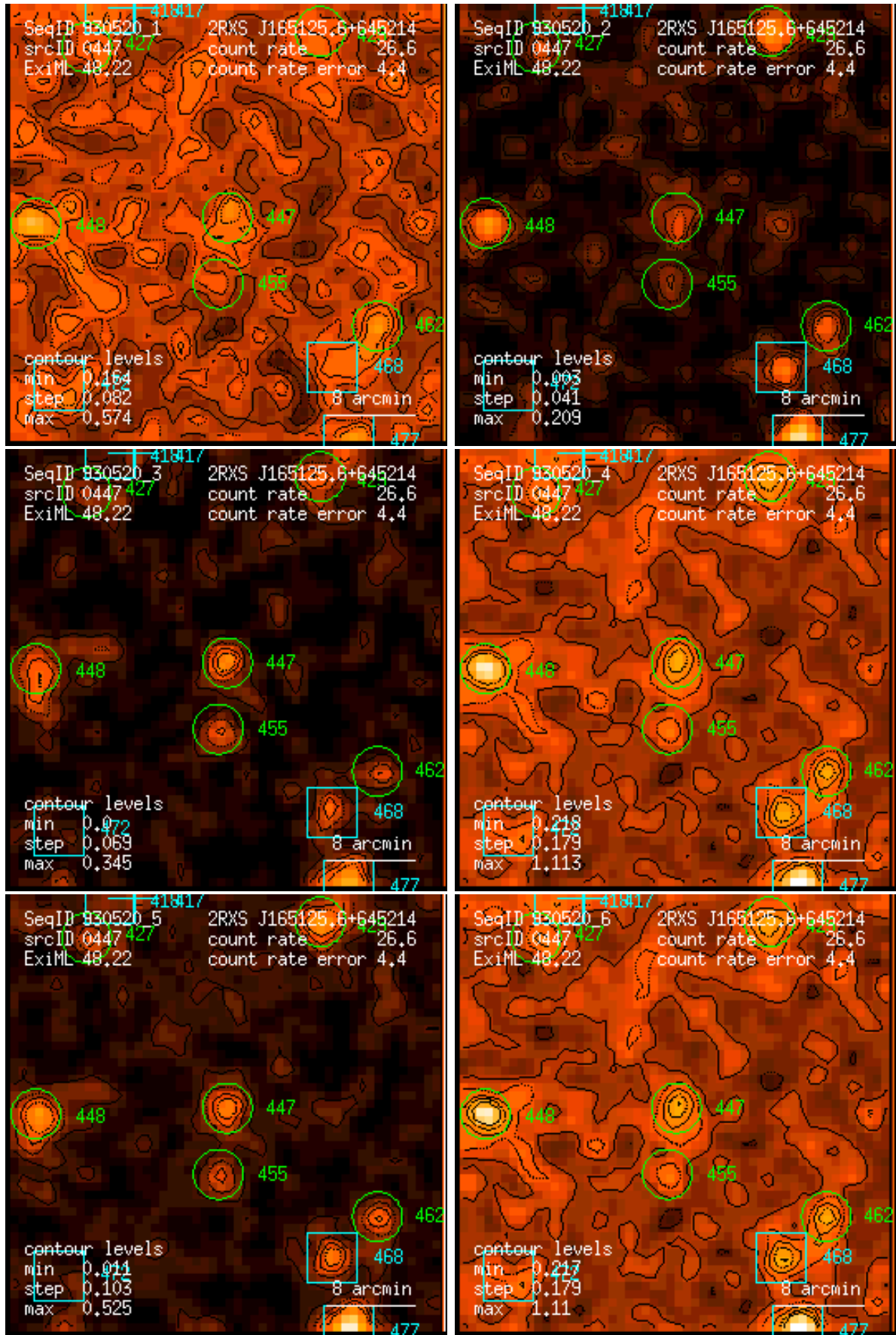
Figure 447: RASS 930520: detection 0447: band rate images, Gaussian filter: (1) PSPC channels 11 – 41, (2) 52 – 90, (3) 91 – 201, (4) 11 – 235, (5) 52 – 201, (6) 11 – 201. Broad band rates in counts/ks. Band rate contour levels in counts/ks/arcmin 2 .
