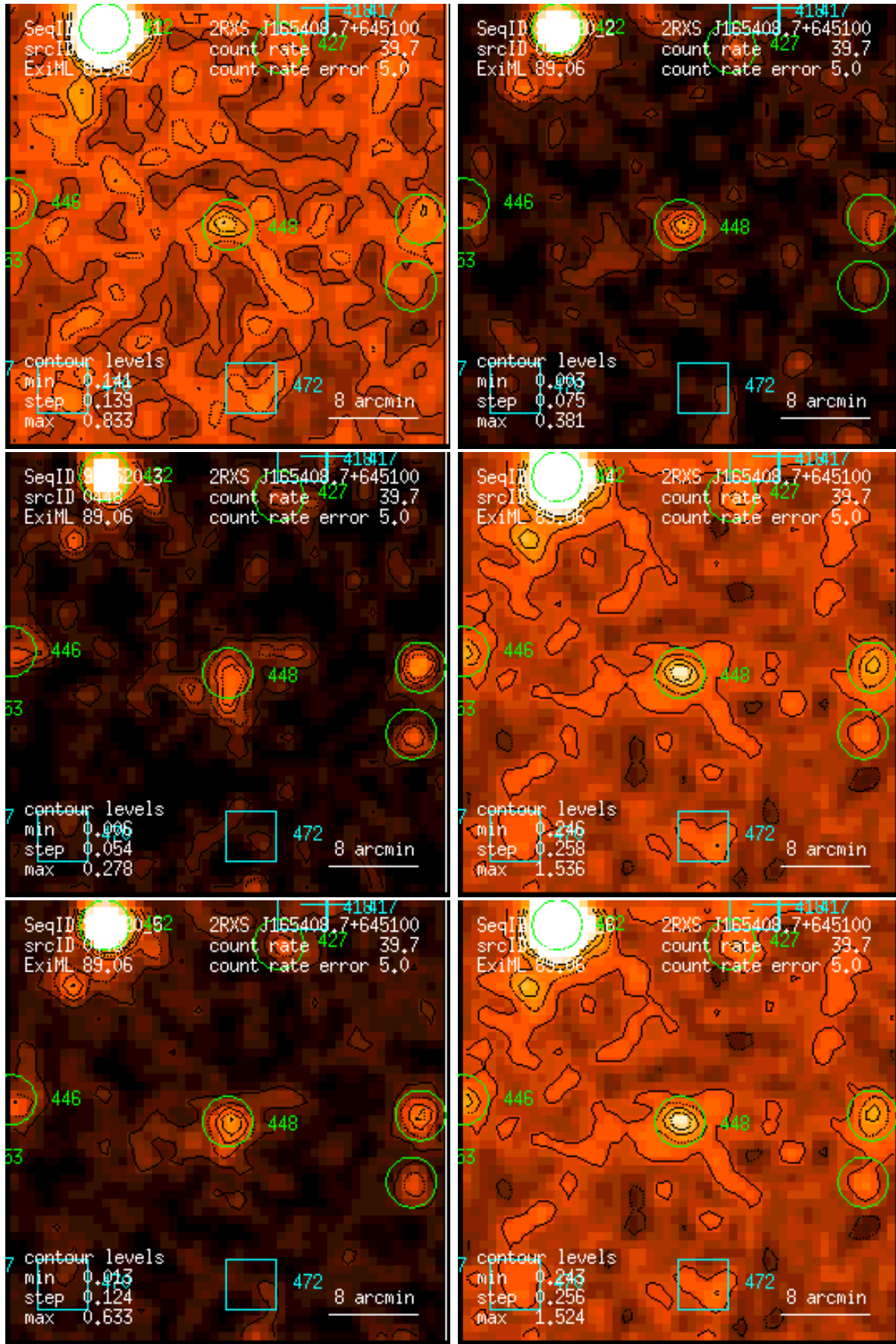
Figure 448: RASS 930520: detection 0448: band rate images, Gaussian filter: (1) PSPC channels 11 – 41, (2) 52 – 90, (3) 91 – 201, (4) 11 – 235, (5) 52 – 201, (6) 11 – 201. Broad band rates in counts/ks. Band rate contour levels in counts/ks/arcmin 2 .
