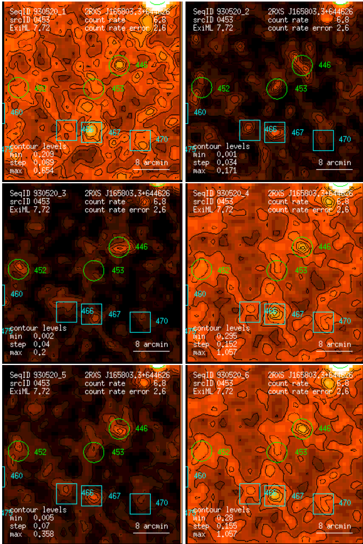
Figure 453: RASS 930520: detection 0453: band rate images, Gaussian filter: (1) PSPC channels 11 – 41, (2) 52 – 90, (3) 91 – 201, (4) 11 – 235, (5) 52 – 201, (6) 11 – 201. Broad band rates in counts/ks. Band rate contour levels in counts/ks/arcmin 2 .
