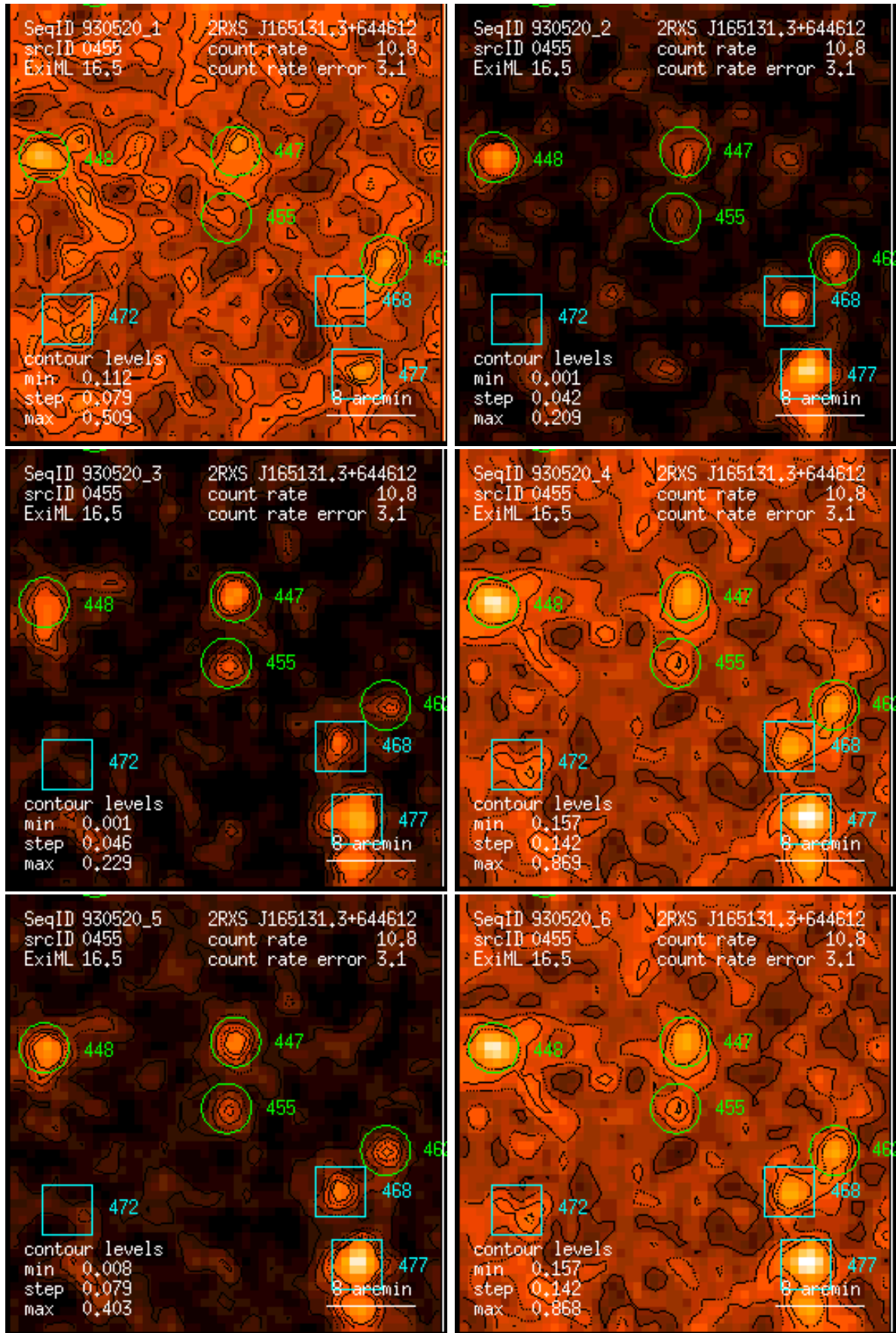
Figure 455: RASS 930520: detection 0455: band rate images, Gaussian filter: (1) PSPC channels 11 – 41, (2) 52 – 90, (3) 91 – 201, (4) 11 – 235, (5) 52 – 201, (6) 11 – 201. Broad band rates in counts/ks. Band rate contour levels in counts/ks/arcmin 2 .
